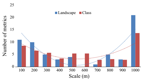
Fig. 5 Frequency of association with each scale as best for species or guilds of bats for class ( n = 21 ) and landscape ( n = 6 ) metrics. Trend lines (2 polynomial) indicate selection across scales. Class variables were rescaled to be comparable to landscape level variables (21:6; class variables divided by 3.5)
