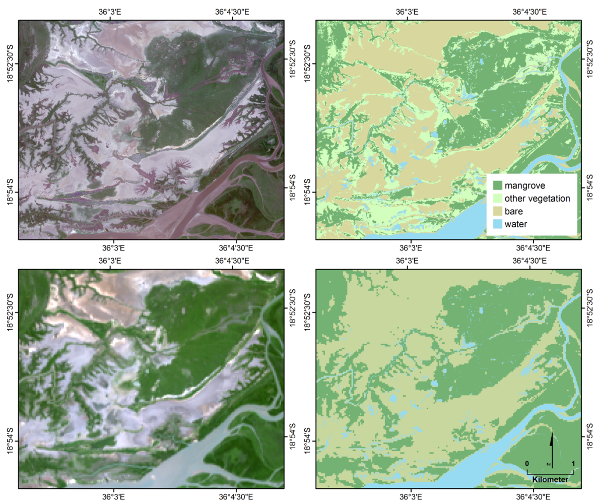
Figure 5. Comparison of mangrove mapping in 2013 with high resolution WorldView-2 ( top row ) and Landsat ( bottom row ) data within the Zambezi River Delta; the satellite image is shown on the left and the classified data on the right.
