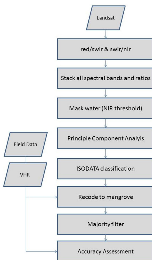
Figure 2. Mapping method for mangrove detection using Landsat, very high resolution (VHR) data and field data.
