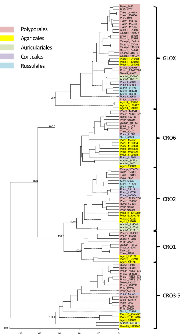
FIG 1 Phylogenetic tree showing relationships among predicted CRO proteins derived from representative white rot fungi, including P. cinnabarinus and P. chrysosporium . ClustalW alignments and tree construction followed the manual deletion of secretion signals and, in the case of CRO3 to CRO5, the removal of repetitive N-terminal WSC domains. On the basis of 1,000 trials, bootstrap values are shown at key nodes. Substitutions were calculated by use of the Kimura distance formula. Taxonomic orders are highlighted by colored shading. Trave, Trametes versicolor ; Dicsq, Dichomitus squalens ; Gansp, a Ganoderma sp.; Phaca, Phanerochaete carnosa ; Bjead, Bjerkandera adusta ; Phlbr, Phlebia brevispora ; Pci and Pycci, Pycnoporus cinnabarinus ; Pleos, Pleurotus ostreatus ; Agabi, Agaricus bisporus ; Aurde, Auricularia delicata ; Punst, Punctularia strigozonata ; Stehi, Stereum hirsutum .
