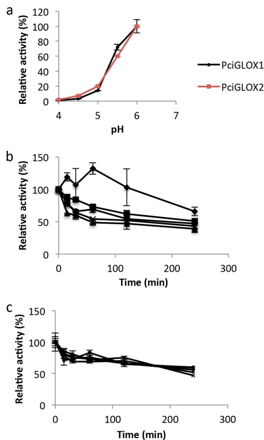
FIG 3 (a) Effect of pH on activity of purified PciGLOX1 and PciGLOX2 . Relative activity represents a percentage of the activity at the maximum pH. (b, c) Effect of pH 4 (◆), pH 4.5 (■), pH 5 (▲), pH 5.5 (×), and pH 6 (●) on the enzymatic stability of PciGLOX1 (b) and PciGLOX2 (c) after different incubation periods. The relative activity after incubation for each pH condition was calculated as a percentage of the activity at the same pH without incubation.
