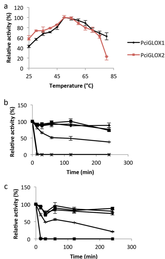
FIG 4 (a) Effect of temperature on enzymatic activity of PciGLOX1 and PciGLOX2 . Values were calculated as a percentage of the activity at the maximum temperature. (b, c) The protein stability of PciGLOX1 (b) and PciGLOX2 (c) at 30°C (◆), 40°C (■), 50°C (▲), 60°C (+), 70°C (*), and 80°C (●) after incubation for different periods of time is represented as a percentage of the activity at 30°C without incubation.
