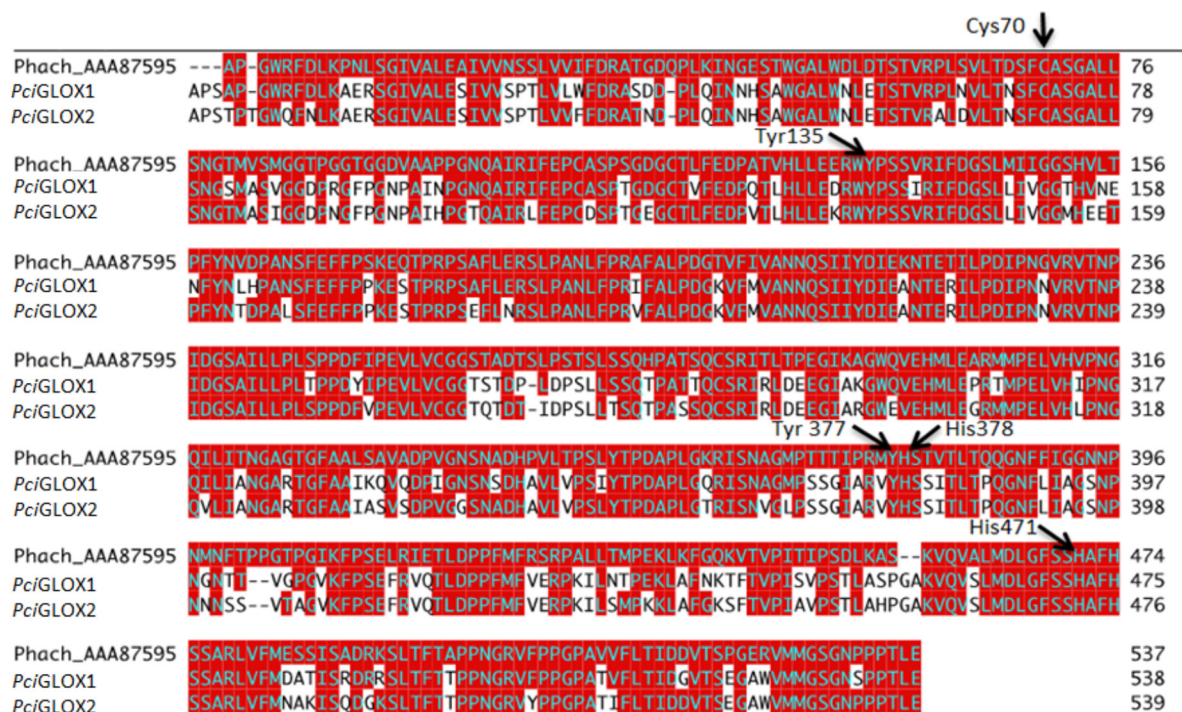
FIG 2 ClustalW alignment of highly expressed Pycnoporus cinnabarinus ( Pci ) GLOX-like proteins with P. chrysosporium ( Phach ) GLOX. Identical residues are highlighted in red. Arrows, residues essential for catalysis.
