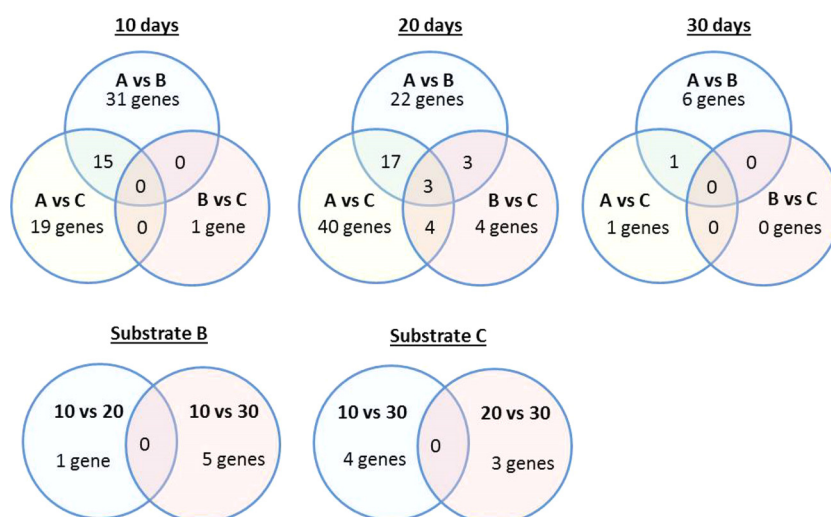
FIG 3 Venn diagrams illustrating the partitioning of P. chrysosporium misregulated genes displaying \geq 2 -fold change when grown on three different poplar substrates. Letters denote substrates (A, B, and C), and numbers refer to time points (10, 20, and 30 days).
