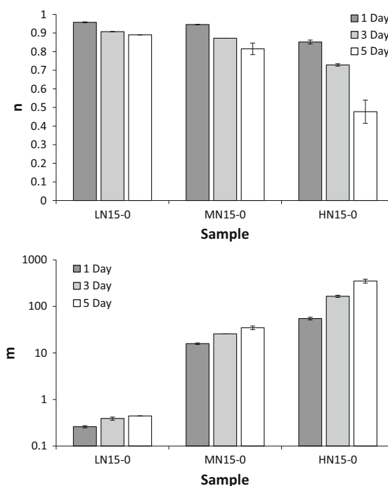
Fig. 3 Values of power law exponent ( n ) and consistency index ( m ) for neat PVA solutions
