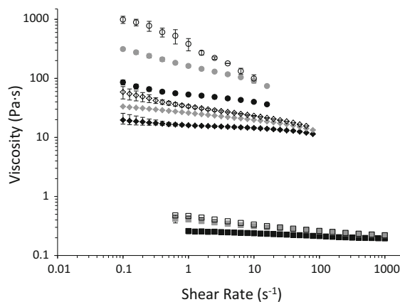
Fig. 2 Shear viscosity data for LN15-0 (square), MN15-0 (diamond), and HN15-0 (circle) at 1 day (black), 3 day (gray), and 5 day (open) aging points. Little aging behavior was seen at the lowest molecular weight while more significant aging was seen at the higher molecular weights as well as more significant shear thinning behavior at high shear rates
