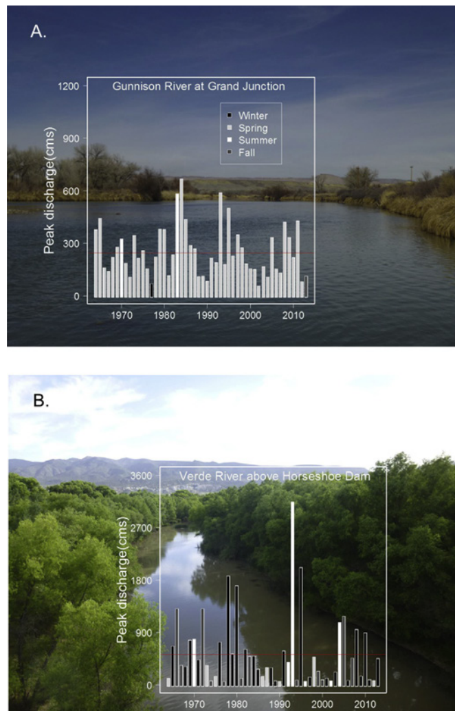
Fig. 3. Examples of variation in magnitude and timing of peak discharge at a Southern Rockies stream (A) and a Central Highland stream (B). Red lines indicate long-term means (1960–2011). (For interpretation of the references to colour in this figure legend, the reader is referred to the web version of this article.)
