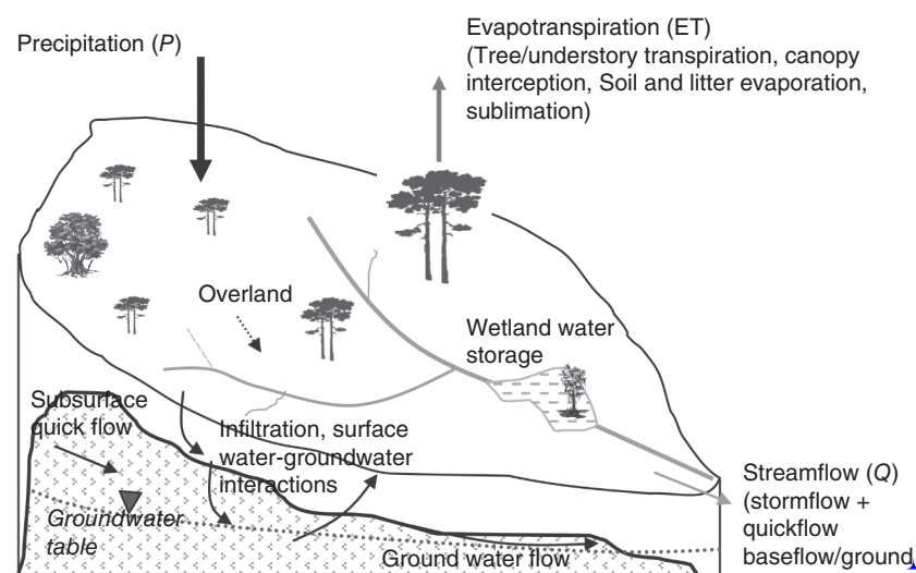
Figure 85.1 A schematic of major hydrologic processes in an undisturbed forest watershed.
