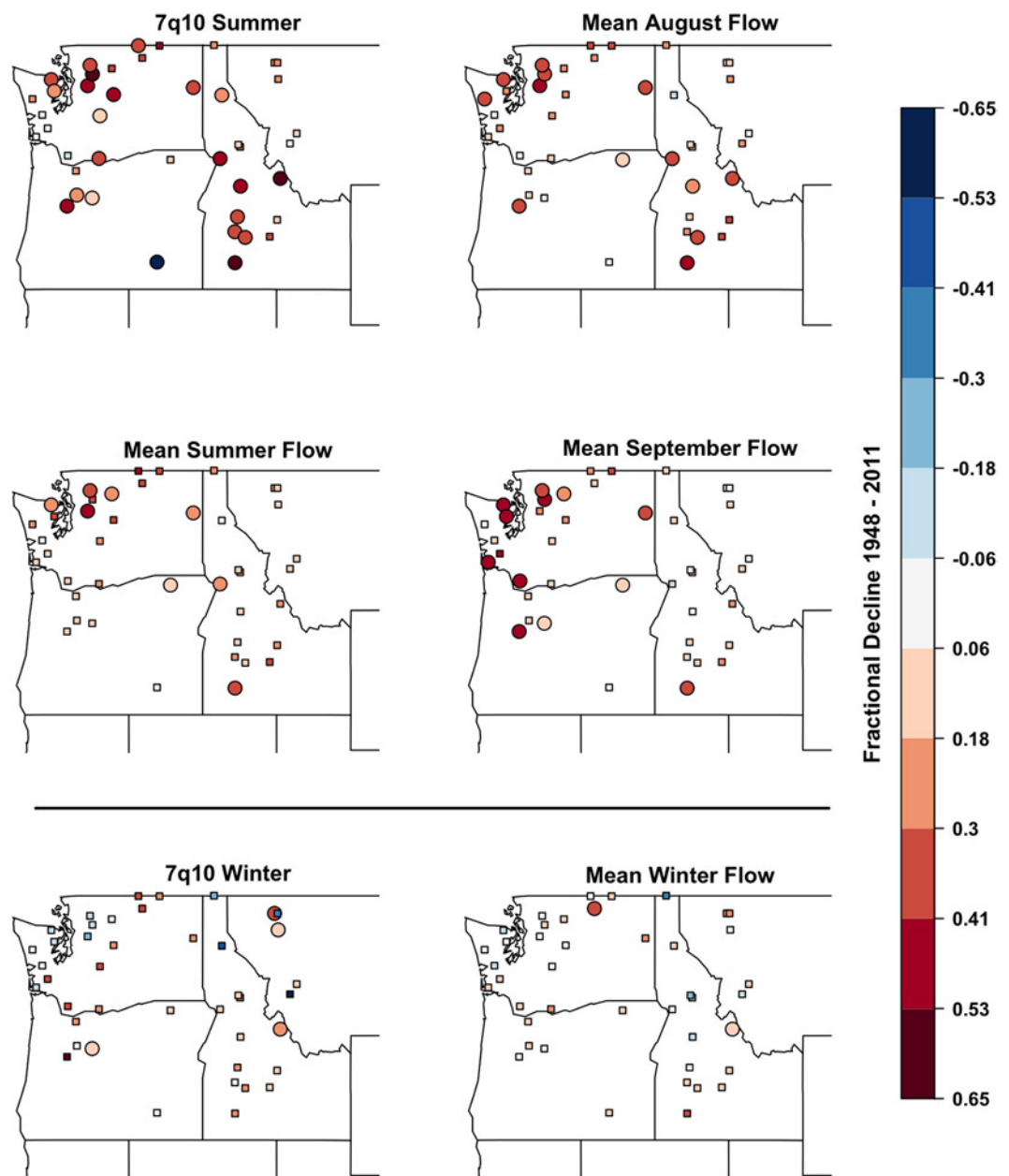
Figure 4. Maps showing mean trends and significance of low flow statistics. Larger circles depict that the trend is significant at the \alpha = 0.10 level.
