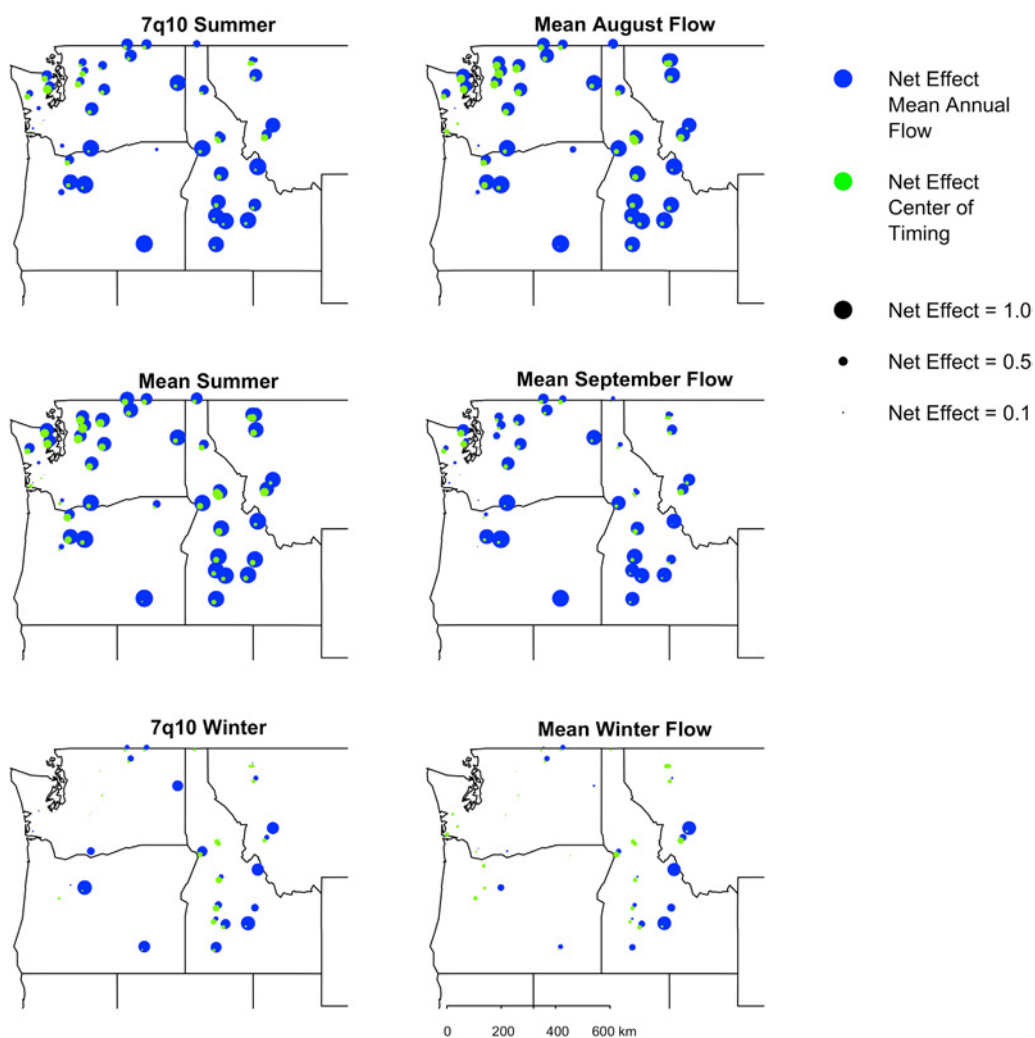
Figure 7. Maps showing the net effect of mean annual streamflow (blue dots) and center of timing (green dots) on low flow metrics. The size of the dots is proportional to the net effect.
