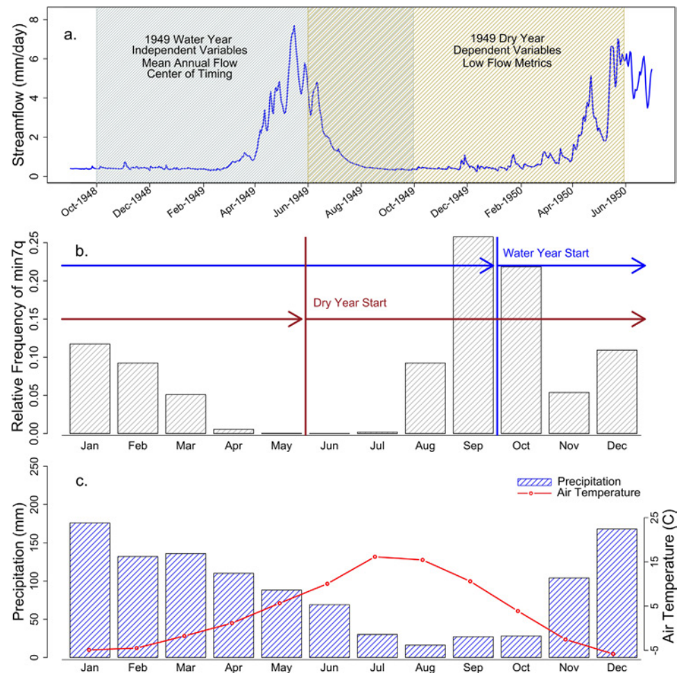
Figure 1. (a) A typical Pacific Northwest hydrograph characterized by snowmelt events showing the water year and dry year, and (b) a relative frequency distribution of the timing of low flow events showing a binomial distribution with the largest peak centered on September and October. Blue lines show the division between water years, which occurs at the peak of low flow. Figure 1c shows typical monthly precipitation and air temperatures showing that times of increased precipitation and air temperature are out of phase.
