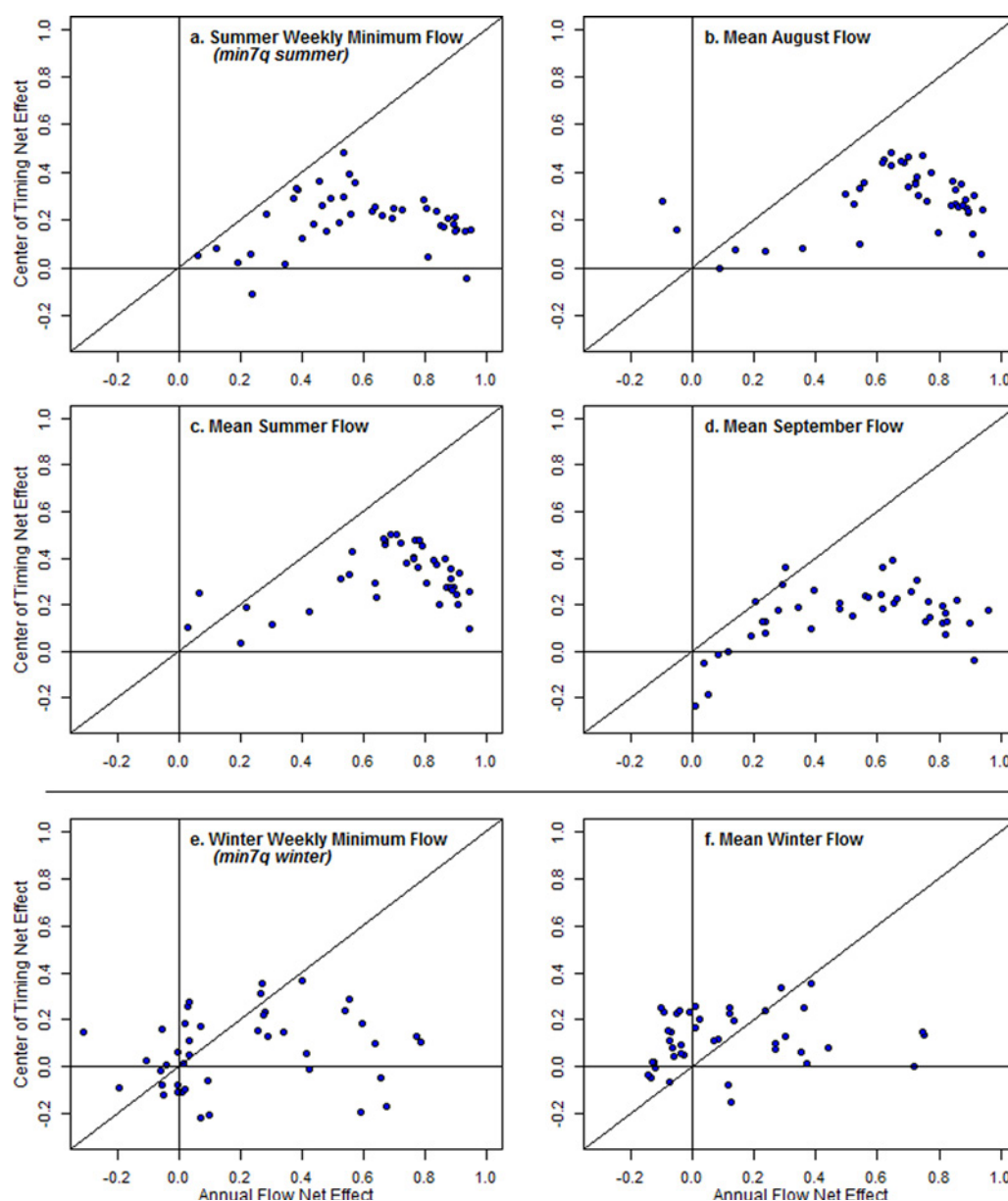
Figure 5. Net effect of mean annual streamflow and center of timing on low flow metrics at each gauge. Points falling on the 1:1 line would be equally affected by amount and timing of streamflow.
