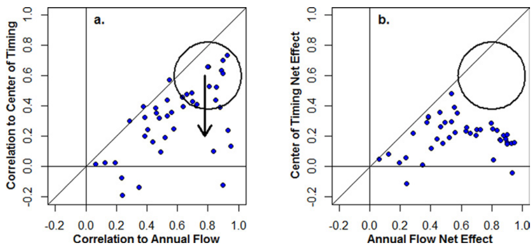
Figure 6. Scatter plots of (a) correlations and (b) net effects of mean annual streamflow and center of timing on min7q summer showing the importance of accounting for the correlation between variables.
