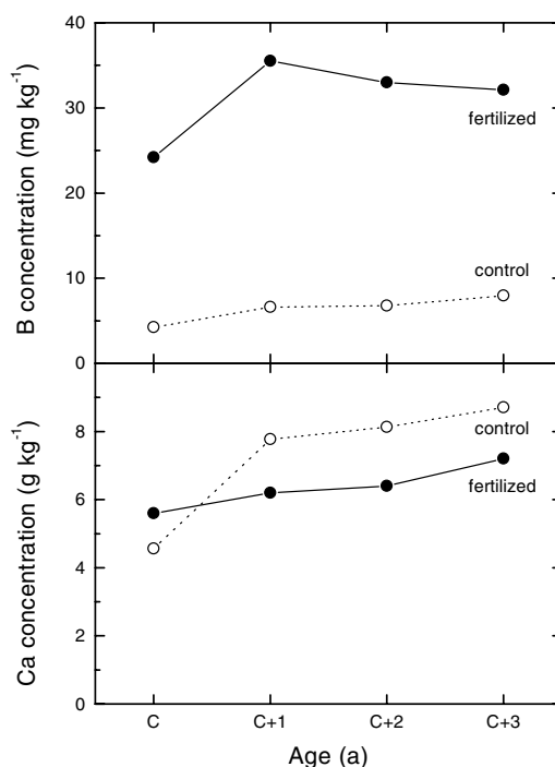
Fig. 2. Changes in boron (B) and calcium (Ca) concentrations in Norway spruce needles with needle age. Sampled in February 1991, from the upper crown and southern exposure. Fertilized with 1.5 \text{ kg ha}^{-1} of B in June 1989, applied as borax. Drawn from data of Lehto and Mälikönen (1994). Data points are means from two plots. Boron: S.E. \leq 4.6 mg kg -1 . Calcium: S.E. \leq 0.93 g kg -1 .
