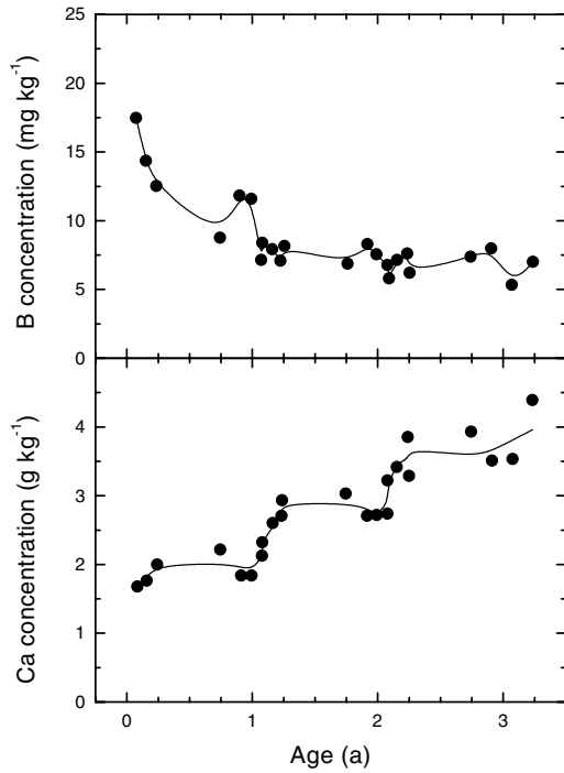
Fig. 3. Changes in boron (B) and calcium (Ca) concentrations in Scots pine needles with needle age. Sampled on three needle classes between June 1983 and September 1984, from a pole stage stand. Lines are B-splines. Redrawn from data in Helmisaari (1990b). Data points are means of 5 to 24 trees. Boron: S.E. \leq 2.6 \text{ mg kg}^{-1} . Calcium: S.E. \leq 0.6 \text{ g kg}^{-1} , except for measurements taken in September for which S.E. \leq 1.4 \text{ g kg}^{-1} .
