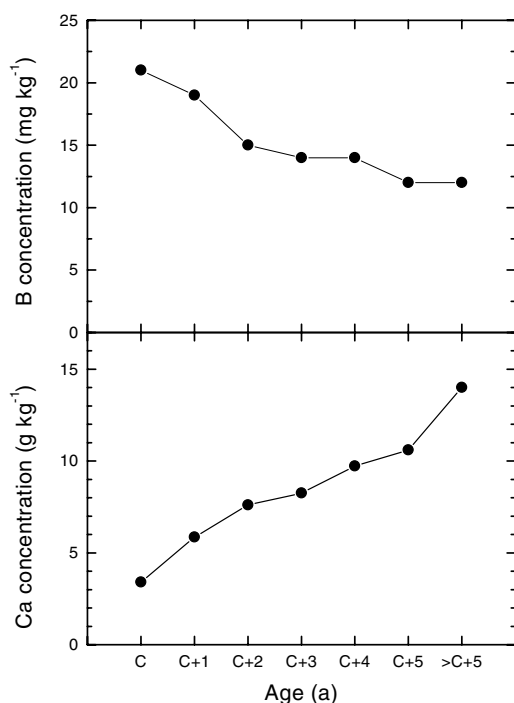
Fig. 1. Changes in boron (B) and calcium (Ca) concentrations in Norway spruce needles with needle age. Sampled in winter 1985, seven branches spanning the whole crown, per each of nine unfertilized trees. Drawn from data of (Finér (1989), Appendix 24). Data points are means. Boron: S.E. \leq 2.3 mg kg -1 . Calcium: S.E. \leq 1.26 g kg -1 .
