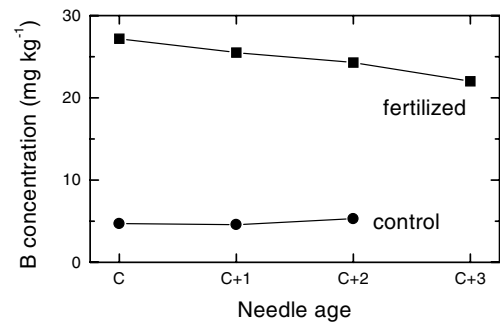
Fig. 5. Changes in boron (B) concentration in Monterey pine needles with needle age. Sampling from the middle crown, in June, six years after fertilization with borax. Means of 4 trees. Drawn from data of Hopmans and Clerehan (1991).
