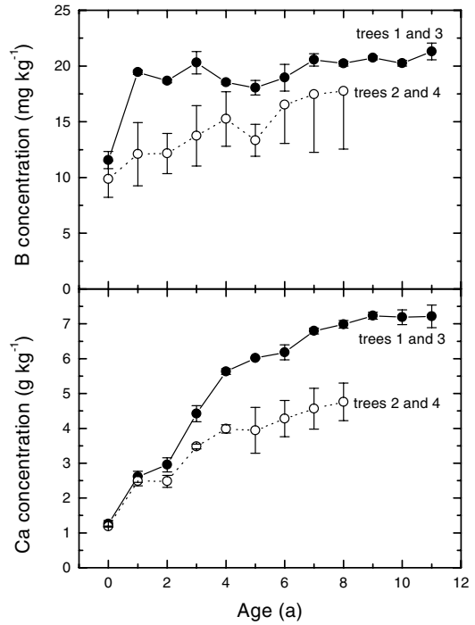
Fig. 4. Changes in boron (B) and calcium (Ca) concentrations in lodgepole pine needles with needle age. Means of two trees \pm S.E. Sampling date was August 1987. Two branches (N and S exposure) from the middle crown of each tree from an 80-year old monospecific stand near Fox Park, Wyoming, U.S.A. Site described by Schoettle and Smith (1999) and analysis methods by Barrick and Schoettle (1996).
