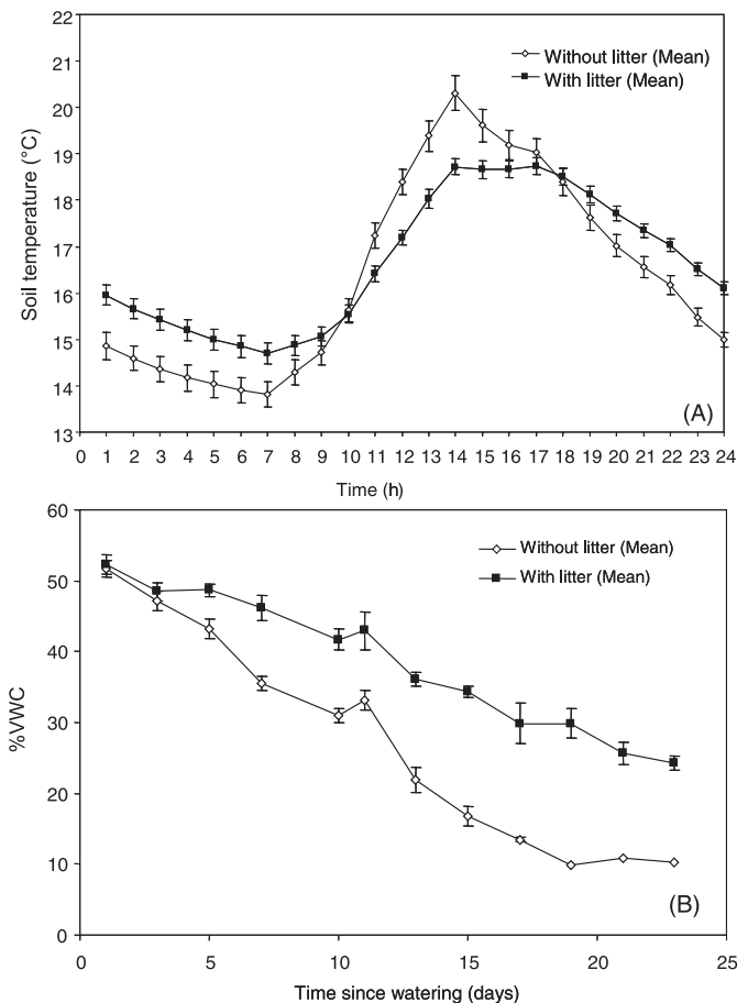
Fig. 4. Effect of scorched litter on the surface of burned soil on soil temperature and moisture during a period of soil drying. (A) Time course of soil temperature ( \pm SE) at 1 cm depth in burned soil with or without scorched litter on top ( N = 10 per
