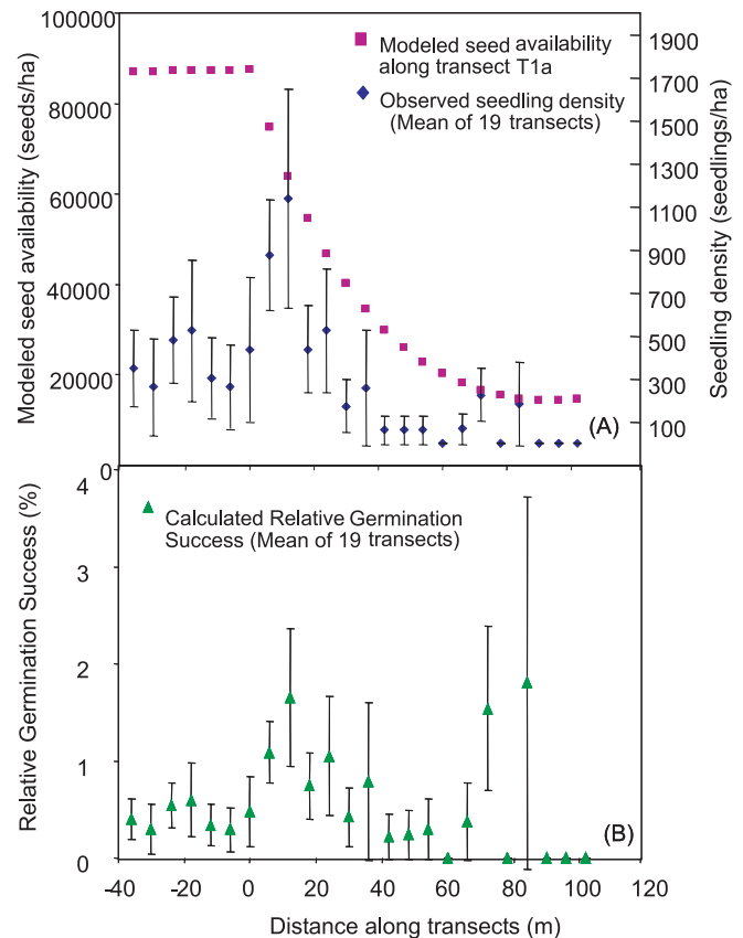
Fig. 3. Spatial distributions of observed seedling density, modeled seed availability, and the calculated variable relative germination success. (A) Observed seedling density ( \pm SE) and an example of the modeled seed availability along one transect (T1a) for each plot receiving seeds from the two opposite sources along transects (see text) and (B) Calculated Relative Germination Success in relation to distance along transects.
