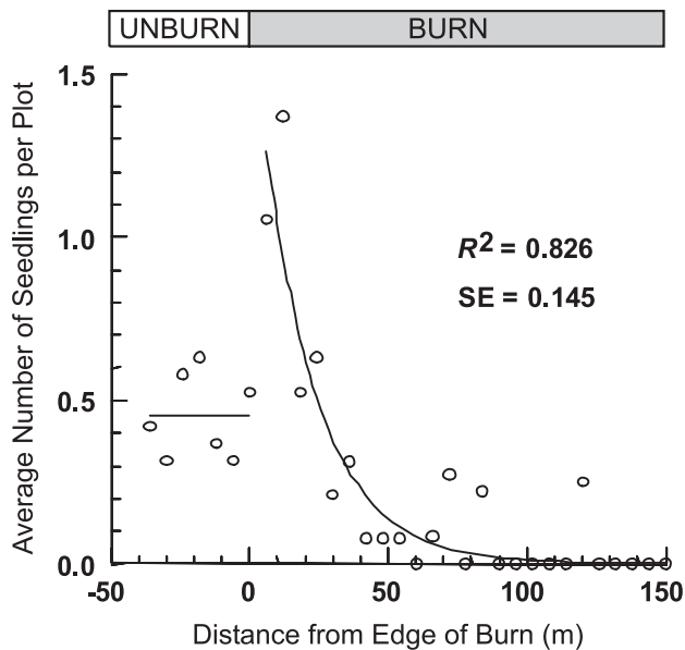
Fig. 2. Mean number of seedlings per 2 m × 6 m plot in June 2002 as a function of distance from the edge of the forest with unburned crowns. Each point is the mean of plots at that position for the 19 transects.
