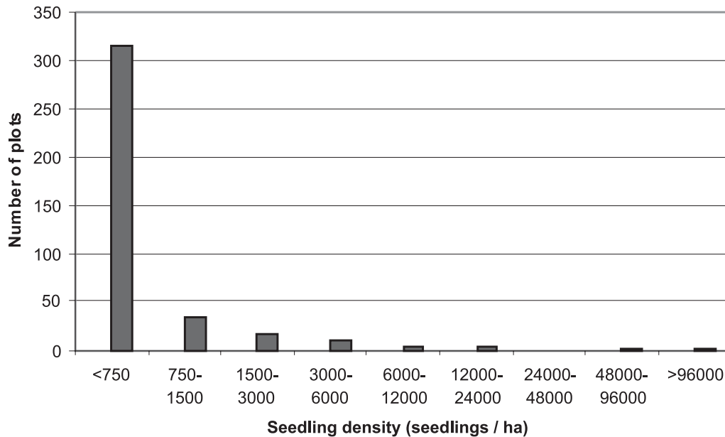
Fig. 1. Distribution of sampled plots by seedling density class for all 20 transects.
