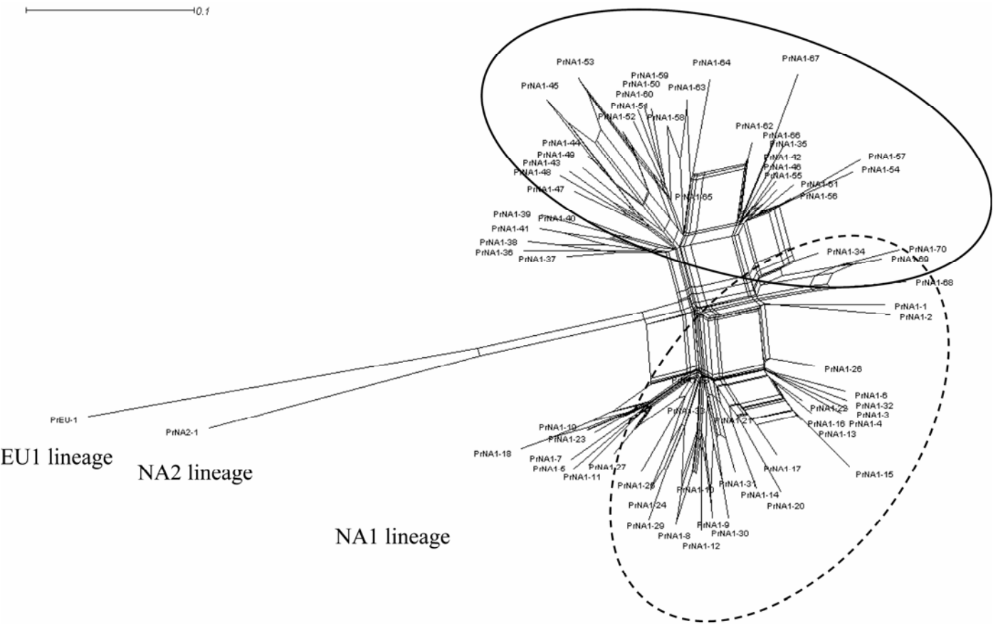
Fig. 3. Split network based on Cavalli-Sforza and Edwards (10) genetic distance of the 72 multilocus genotypes detected in the Phytophthora ramorum population on the West Coast of the United States. The solid line encompasses the approximate position of genotypes unique to the Oregon forest population, whereas the broken line encompasses the approximate position of genotypes unique to the California or Washington populations.
