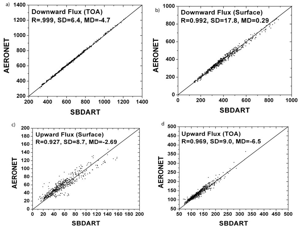
Figure 2. Upward and downward SW fluxes at the surface and TOA from the AERONET inversion product as a function of upward and downward SW fluxes at the surface and TOA from SBDART calculations.
