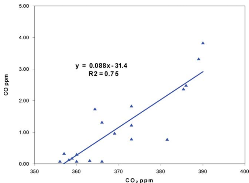
Figure 6. Carbon dioxide (CO 2 ) and carbon monoxide (CO) concentrations based on all 2001 aerial samples.
