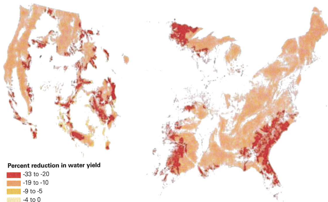
Figure 10.2—Spatial distribution of annual forest water yield response (percent reduction in water yield) to a 10-percent decrease in precipitation across the conterminous United States. Darker shades represent a greater percent reduction relative to lighter shades. Simulation results at the U.S. Geological Survey HUC-8 scale are presented at 1-km resolution by a mask of forest land cover (Source: Sun and others 2015).
