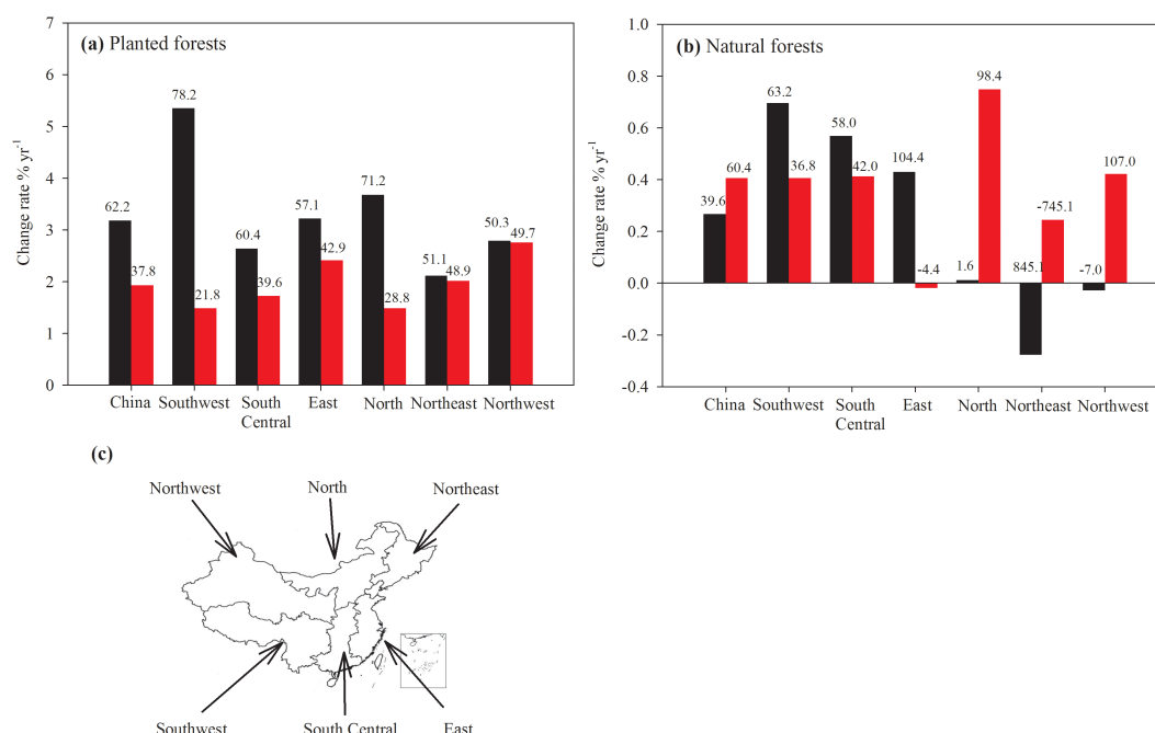
Figure 1. Rate of change and the relative contributions of forest area and biomass density to carbon sinks in planted (a) and natural (b) forests in six broad regions of China for the period 1977–2008. The division of these six broad regions is indicated in (c). Bars and numbers above represent the rates of change and the relative contributions of forest area (in black) and carbon density (in red), respectively.
