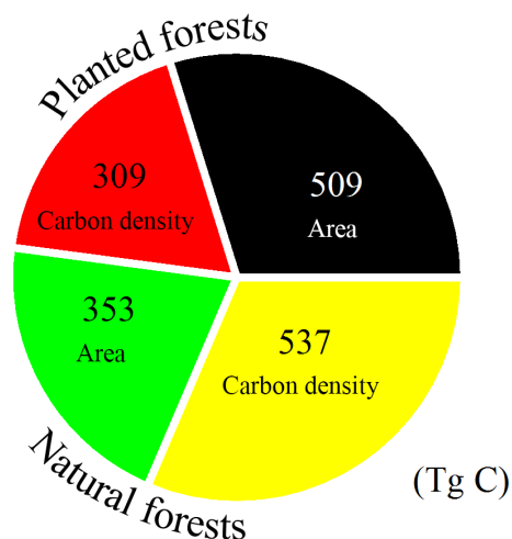
Figure 5. Summary of the forest biomass carbon sinks attributing to areal expansion and increase in carbon density for planted and natural forests of China in the period 1977–2008.
