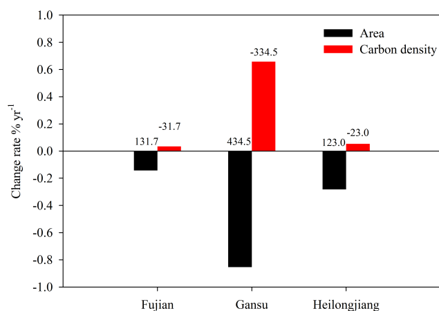
Figure 3. Rate of change and the relative contributions of changes in forest area and carbon density of natural forests to carbon loss in three provinces of China in the period 1977–2008. Bars and numbers above represent the rates of change and the relative contributions of forest area (in black) and carbon density (in red), respectively.
