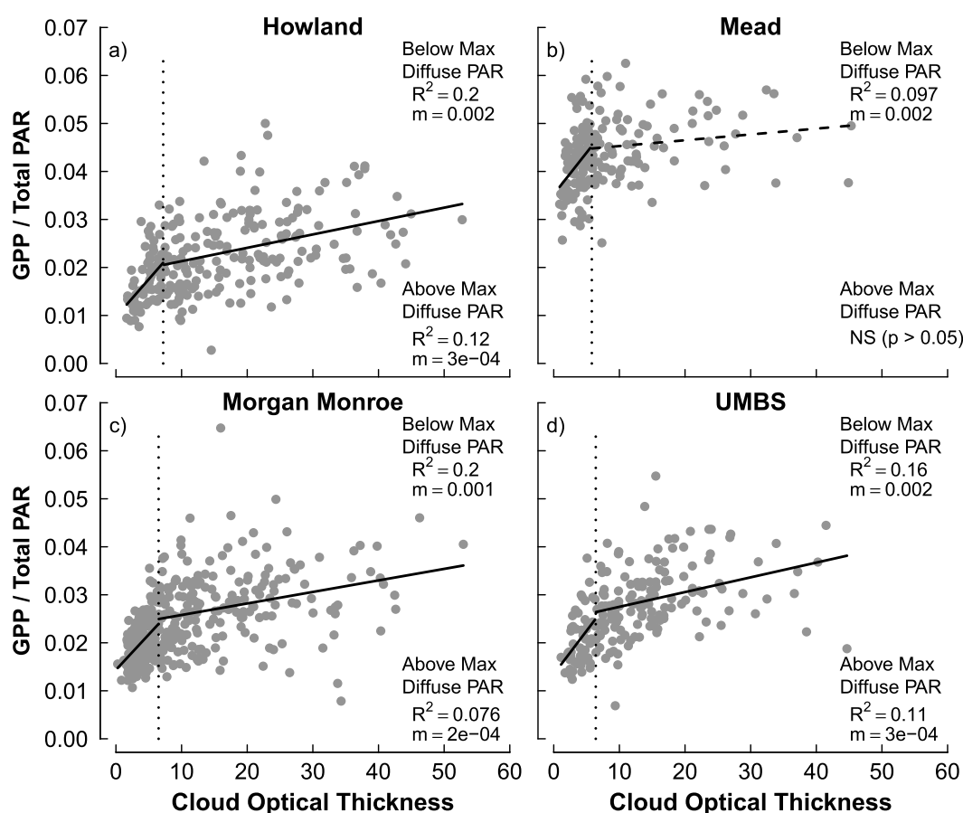
Figure 4. During the peak growing season (average start date and length listed in Table 1), light-use efficiency (gross primary production per unit total PAR) increases with cloud optical thickness ( \tau_c ) at (a) Howland Forest, (b) Mead, (c) Morgan Monroe, and (d) UMBS. The vertical dotted line represents the \tau_c where the maximum diffuse PAR occurs at each site (see Figure 1). The peak growing season only covers a portion of time from May through September, which are shown in Figures 1–3. The dashed regression line in Figure 4b indicates a relationship that is not significant (NS; p > 0.05 ). The solid regression lines shown in all panels indicate relationships with p < 0.01 .
