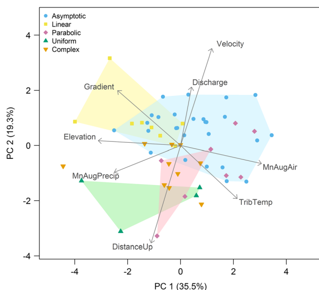
Figure 6. Principal components analysis (PCA) biplot showing the relationship in multivariate space of river temperature profiles (symbols) with respect to the strength and direction of partial correlations between water temperature and hydroclimatic variables (arrows). Note that the ordination is of partial correlation coefficients. Symbols indicate the class to which each profile was assigned. Coloured polygons enclose symbols of the same colour, with blue for asymptotic , yellow for linear , green for uniform and pink for coastal parabolic profiles. Inland parabolic profiles are pink symbols within the blue polygon. Abbreviations: MnAugAir, mean August air temperature; MnAugPpt, mean August precipitation; TribTemp, temperature of tributaries; and DistanceUp, distance upstream
