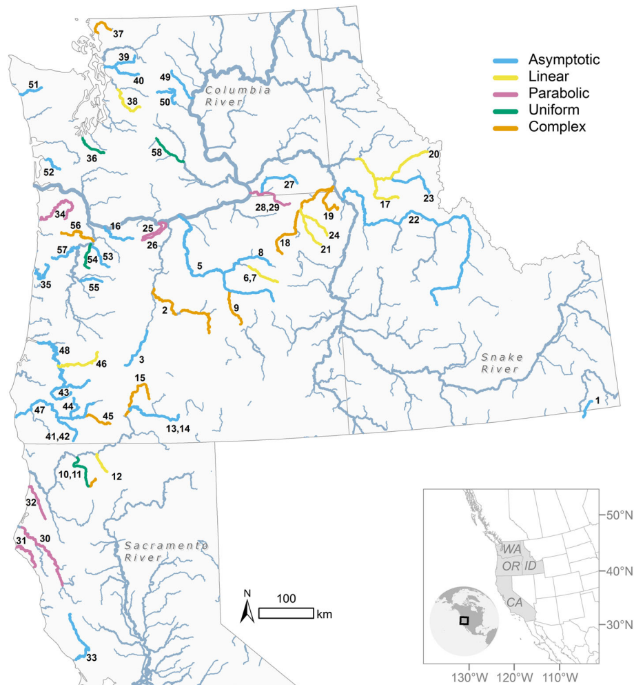
Figure 4. Geographic locations of rivers in each profile class
