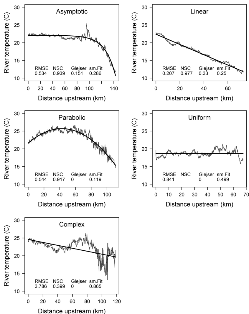
Figure 3. Examples of profile classification and diagnostics for asymptotic , linear , parabolic , uniform and complex profiles. For each example, the plot shows river temperature versus distance surveyed in grey and fitted values for the best model selected from the candidate set in black. Diagnostic goodness of fit metrics root mean square error (RMSE), Nash–Sutcliffe Coefficient (NSC), p -value from a Glejser test for homoscedasticity (Glejser) and the difference in root mean squared error (RMSE) between the best model and a smoothed trend (20-knot GAM; sm. Fit) are shown on each plot. For the complex profile example, diagnostic values refer to the linear fit (solid line); the smoothed fit (dotted line) is also presented to illustrate the trend. The rivers shown are Asymptotic : Little Deschutes River (2001); Linear : Minam River (1999); Parabolic : Mattole River (2001); Uniform : Deschutes River (Puget Sound) (2003); and Complex : Joseph Creek (1999). Plots of other profiles are provided in Figure A2
