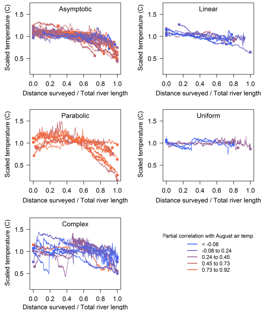
Figure 5. Partial correlations between river temperature and mean August air temperature for longitudinal profiles assigned to each class ( asymptotic , linear , parabolic , uniform and complex ). The longitudinal profiles within each class are standardized on both axes to facilitate comparison of partial correlations among profiles. The downstream (circles) and upstream (squares) end points of individual surveys are demarcated to indicate the extent of the river included in each survey. Non-standardized plots of longitudinal profiles for all rivers assigned to each profile class are provided in Figure A2
