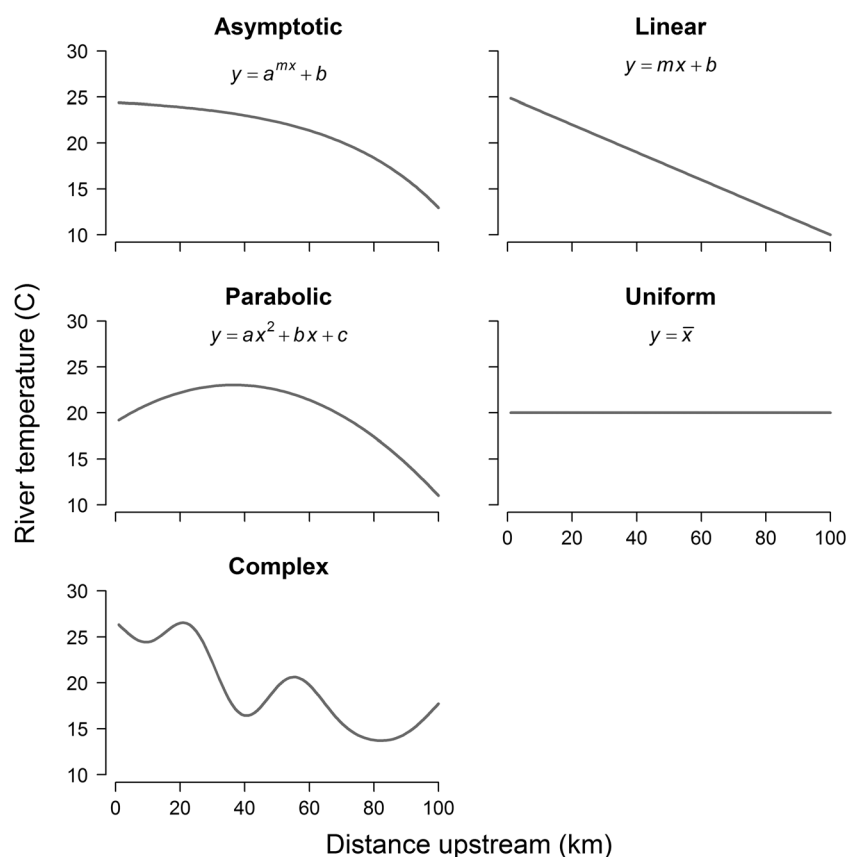
Figure 2. Theoretical representations and model equations for the five thermal profile classes, where y is river temperature ( ^{\circ}\text{C} ), x is the distance upstream from the downstream terminus of the profile (km), and a , b , c and m are constants
