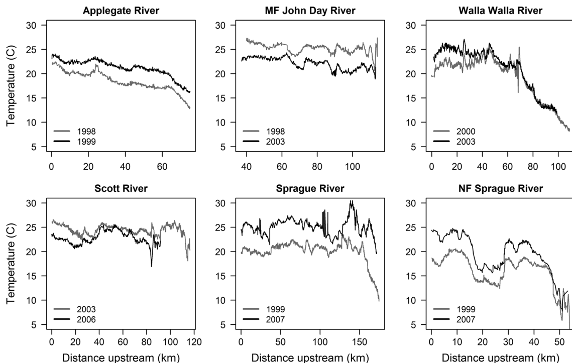
Figure 1. Longitudinal profiles for rivers in which surveys were flown in 2 years, illustrating similar spatial variance patterns. The NF Sprague River did not meet analysis criteria, but we included it here to illustrate consistency among years
