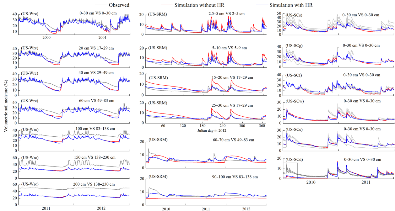
Figure 1. Observed and simulated soil moisture over selected years. Labels at the upper right corner of each soil moisture panel show the depths of observed and simulated soil moisture. For example, “20 cm VS 17–29 cm” means the observation depth of soil moisture is 20 cm and the simulated results at depths of 17–29 cm were compared with this observation. Within panels for southern California sites (US-SCs, US-SCg, US-SCf, US-SCw, US-SCc, and US-SCd), the four grey lines are data from the four CS-616 soil moisture sensors at 0–30 cm depth. Results were shown for the last year only (2012) for the top 30 cm depths at US-SRM site for clarity. The rectangular box indicated period with incomplete precipitation record.
