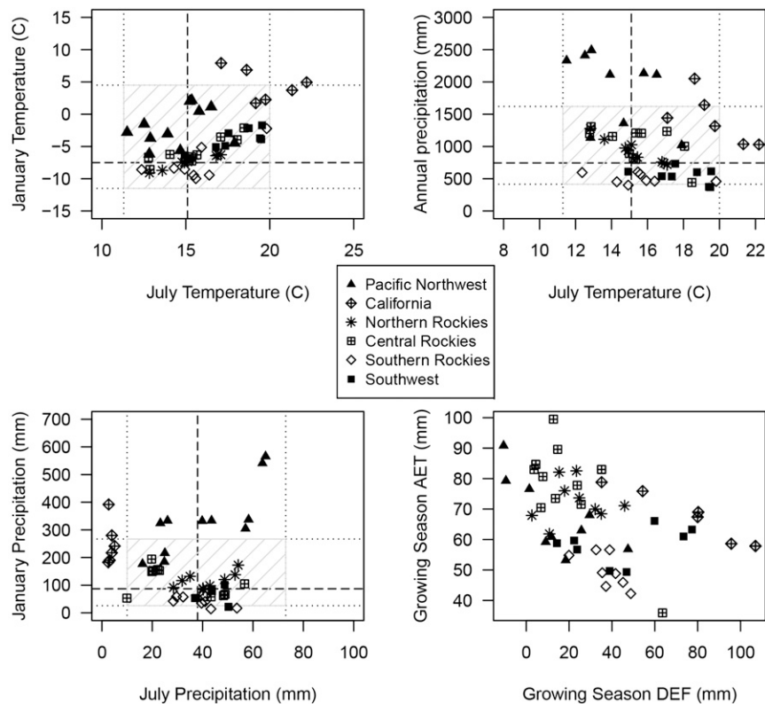
Fig. S1. Distribution of sampling sites in climate space. The climatic limits of Douglas fir (34) are represented as 10th and 90th percentiles (dotted lines) and 50th percentiles (dashed line). The hatched box symbolizes the fundamental climate niche of Douglas fir. Sampling sites are plotted in this climate space based on average values (1916–2006) of the variables indicated. The distribution of sample sites represents the realized climate niche of Douglas fir.
