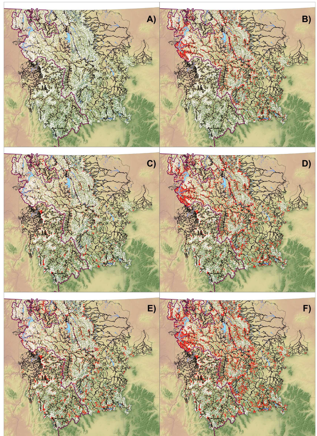
Fig 4. Predictions of 10% PRTA under multiple scenarios. Prediction maps showing whether stream reaches are expected to remain below the classification threshold (0.384) for 10% rainbow trout alleles at a site (stream reaches in black, no; in white, yes). Panel A shows the current scenario and remaining panels show predictions relative to current conditions. Scenarios match those in Table 4 for current (panel A), equilibrium (panel B), current +0.5°C (panel C), equilibrium +0.5°C (panel D), current +1.0°C (panel E), and equilibrium +1.0°C (panel F). Reaches in red are those expected to exceed this threshold relative to the current scenario.
