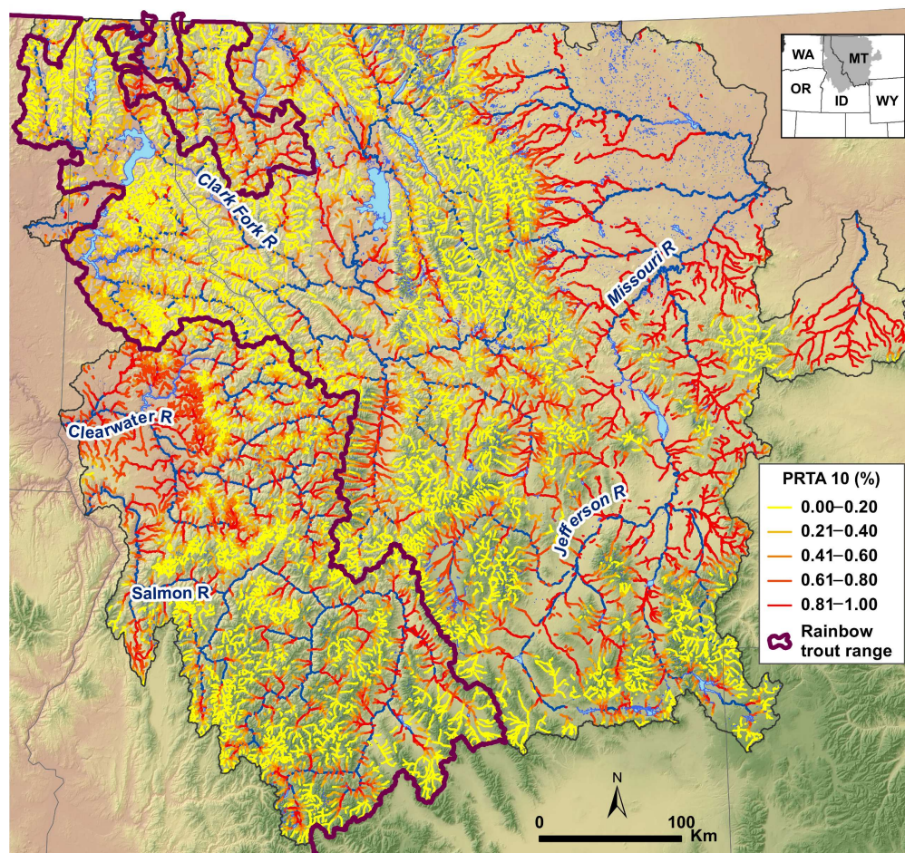
Fig 3. Predictions of 10% PRTA in the study area. Probabilities that the percentage of rainbow trout alleles at a site will exceed 10% (PRTA 10) across the range of westslope cutthroat trout in Montana and Idaho under current conditions. Blue river segments had mean annual flows > 7 \text{ m}^3/\text{s} where model predictions were not made.
