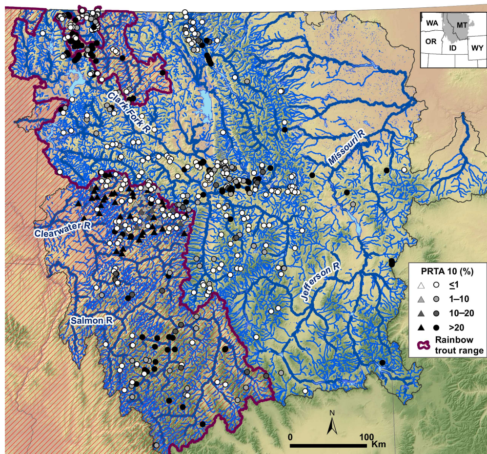
Fig 1. Sites in the synthetic analysis. Study area showing elevation hillshade, stream network, overlap in the historical ranges of rainbow trout and westslope cutthroat trout (purple hashmarks overlaying the stream network), and locations of 558 sample sites, scaled by levels of introgression (<1%, white; 1–10%, light gray; 10–20%, dark gray; >20%, black), used to develop logistic regression models. Most sites ( n = 501 ) provided estimates of the percentage of rainbow trout alleles at a site (PRTA; circles). Some sites ( n = 57 ) provided only estimates of the percentage of fish with rainbow trout alleles (PFRT; triangles). Thick stream lines show rivers with mean annual flows that exceeded 2.83 \text{ m}^3/\text{s} .
