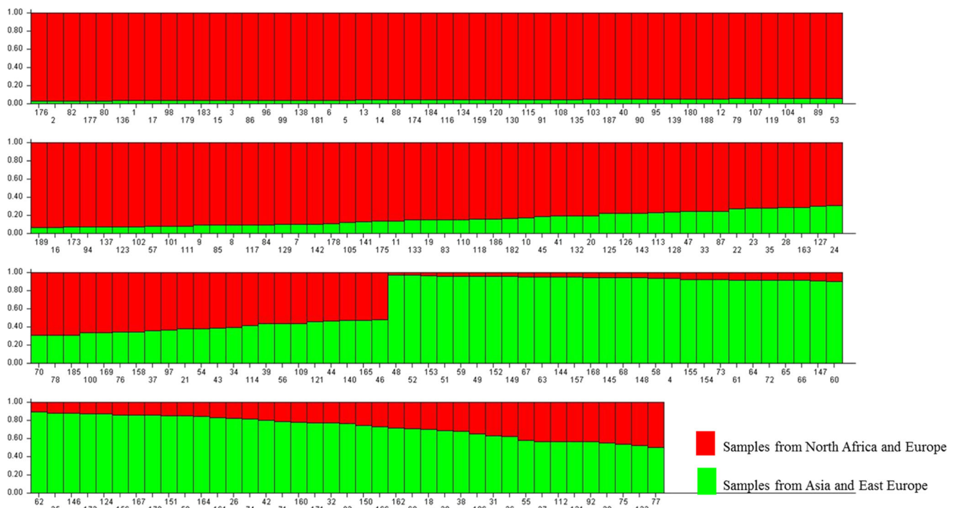
Fig. 2 Population structure of 189 accessions based on 10 SSR markers ( K = 2 ) and graph of estimated membership fraction for K = 2
