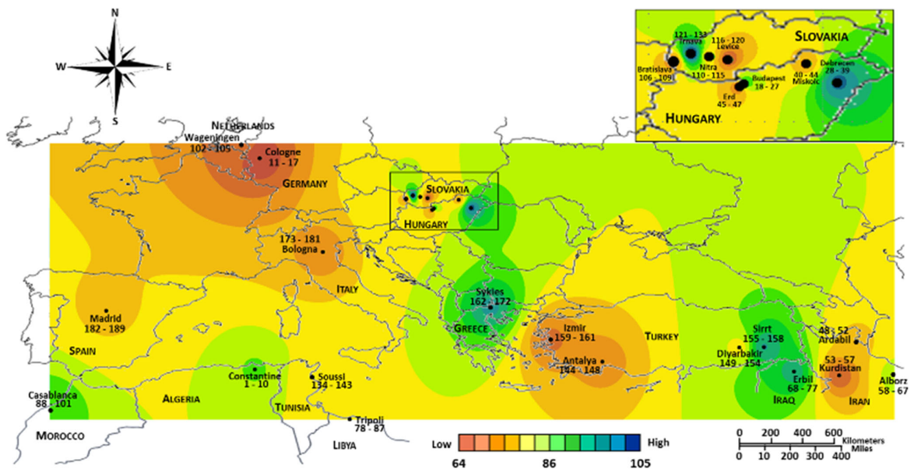
Fig. 1 Geographical variation of allelic richness in J. regia across 14 sampled countries
