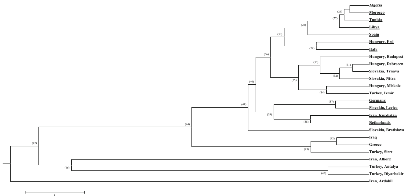
Fig. 4 Neighbor-joining dendrogram of 25 groups of J. regia based on Nei's genetic distance at ten SSR loci
