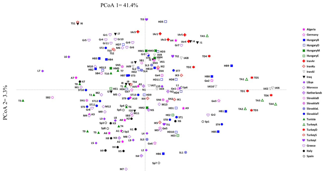
Fig. 5 BiPlot obtained from PCoA analysis of all accessions showing distribution of walnut samples in two main dimensions
