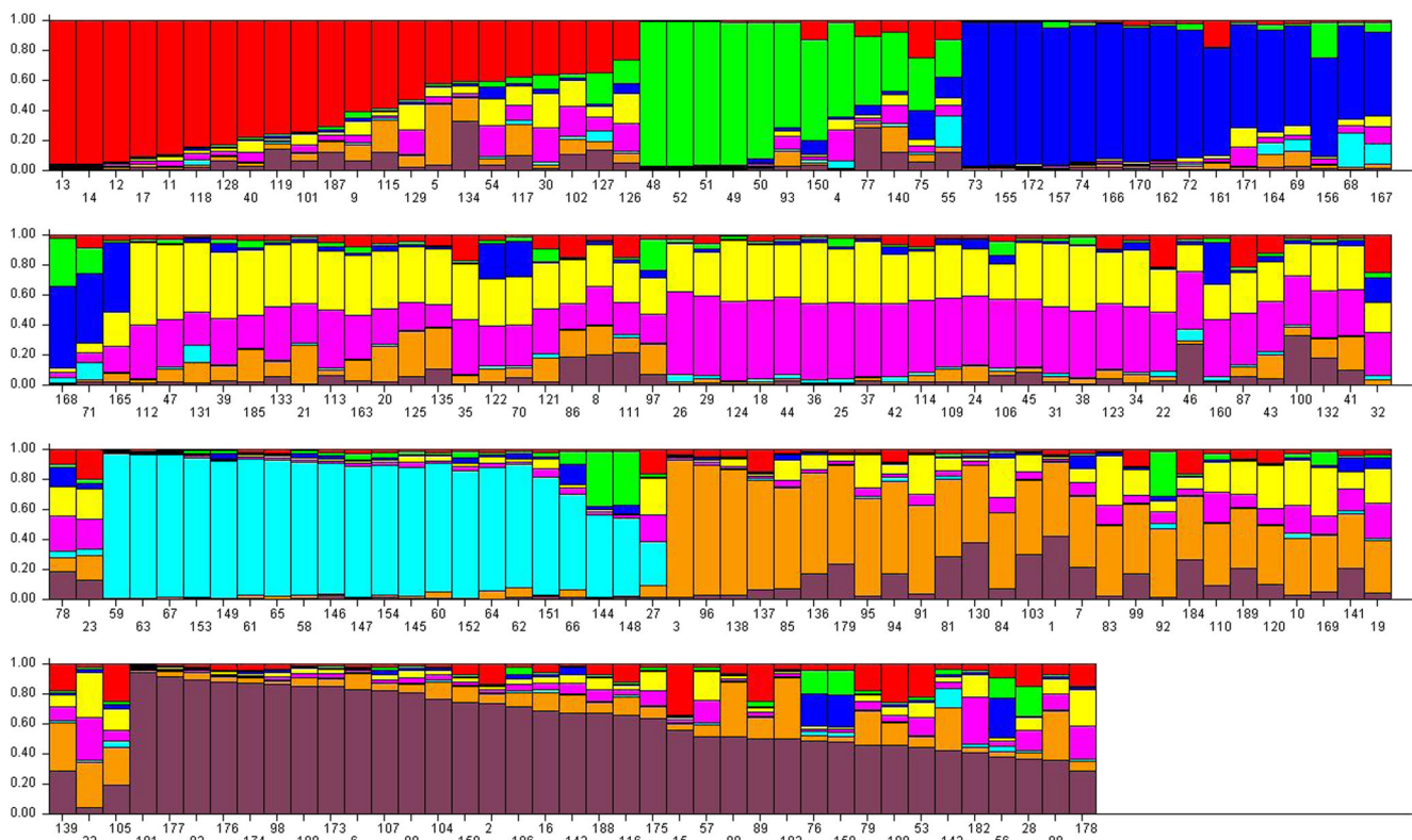
Fig. 3 Population structure of 189 Persian walnut accessions based on ten SSR markers ( K = 8 )
