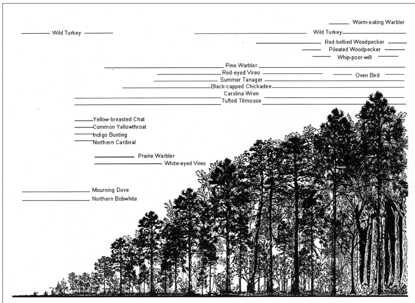
Fig. 4. Plant succession and breeding bird community succession model of selected common species occurrence associated with different stages of succession within shortleaf pine-bluestem forests in the absence of fire. Horizontal lines indicate only the presence of the named species at a particular successional stage. Based on Johnston and Odum (1956), Meyers and Johnson (1978), Engstrom et al. 1984, Wilson et al. (1995), Jennelle (2000), and Masters et al. (2002).
