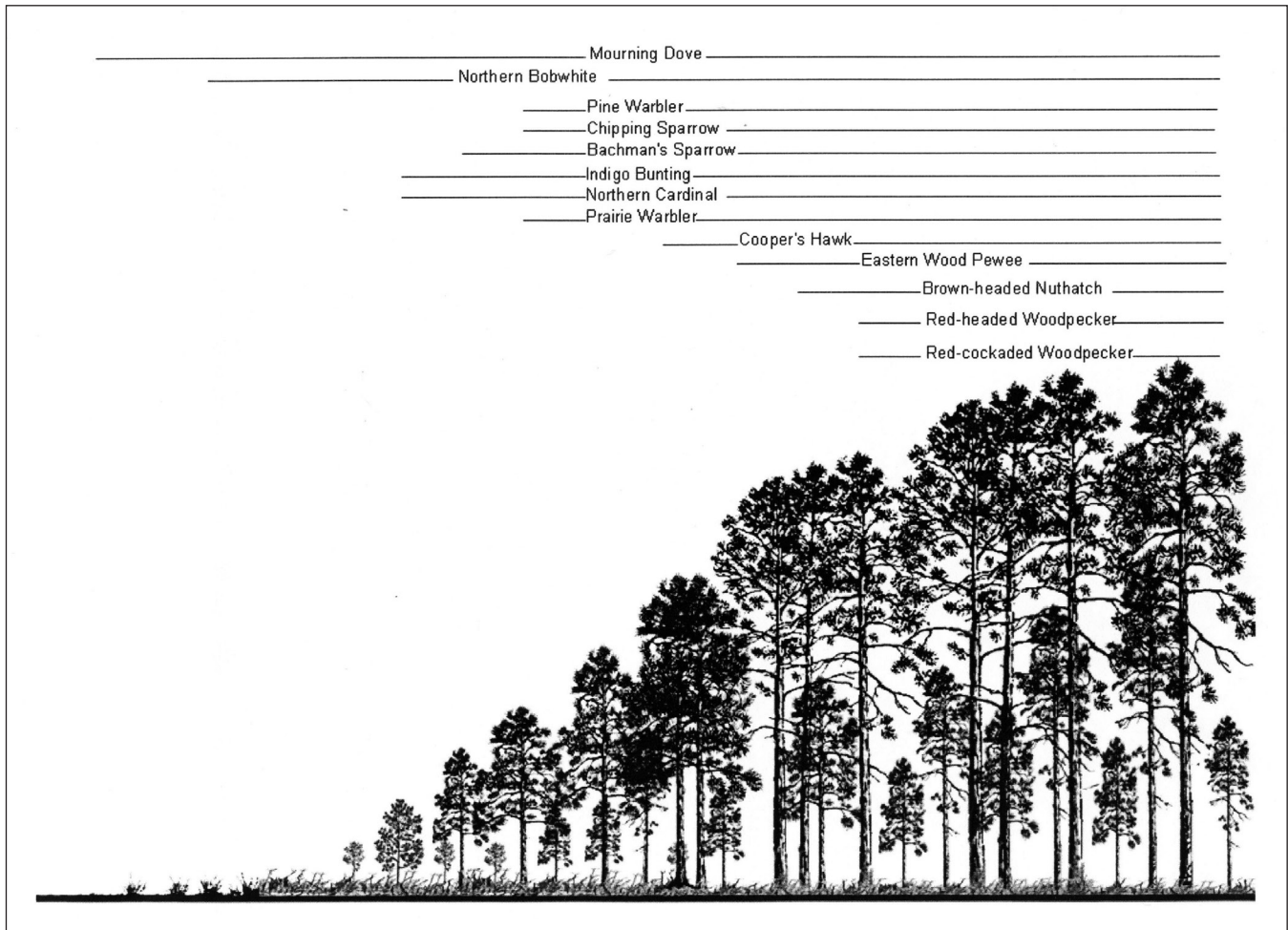
Fig. 5. Plant succession and breeding bird community succession model of selected common species occurrence associated with different stages of succession within shortleaf pine-bluestem forests with frequent fire of at least 1- to 5-year intervals. Most of the bird species from Fig. 4 will be found here as well if even 3.4 m 2 of hardwood basal area per hectare is present in the stand. Horizontal lines indicate only the presence of the named species at a particular successional stage. Based on Wilson et al. (1995), Jennelle (2000), and Masters et al. (2002).
