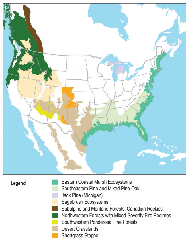
Fig. 1. Map of North American types reviewed in this assessment.
