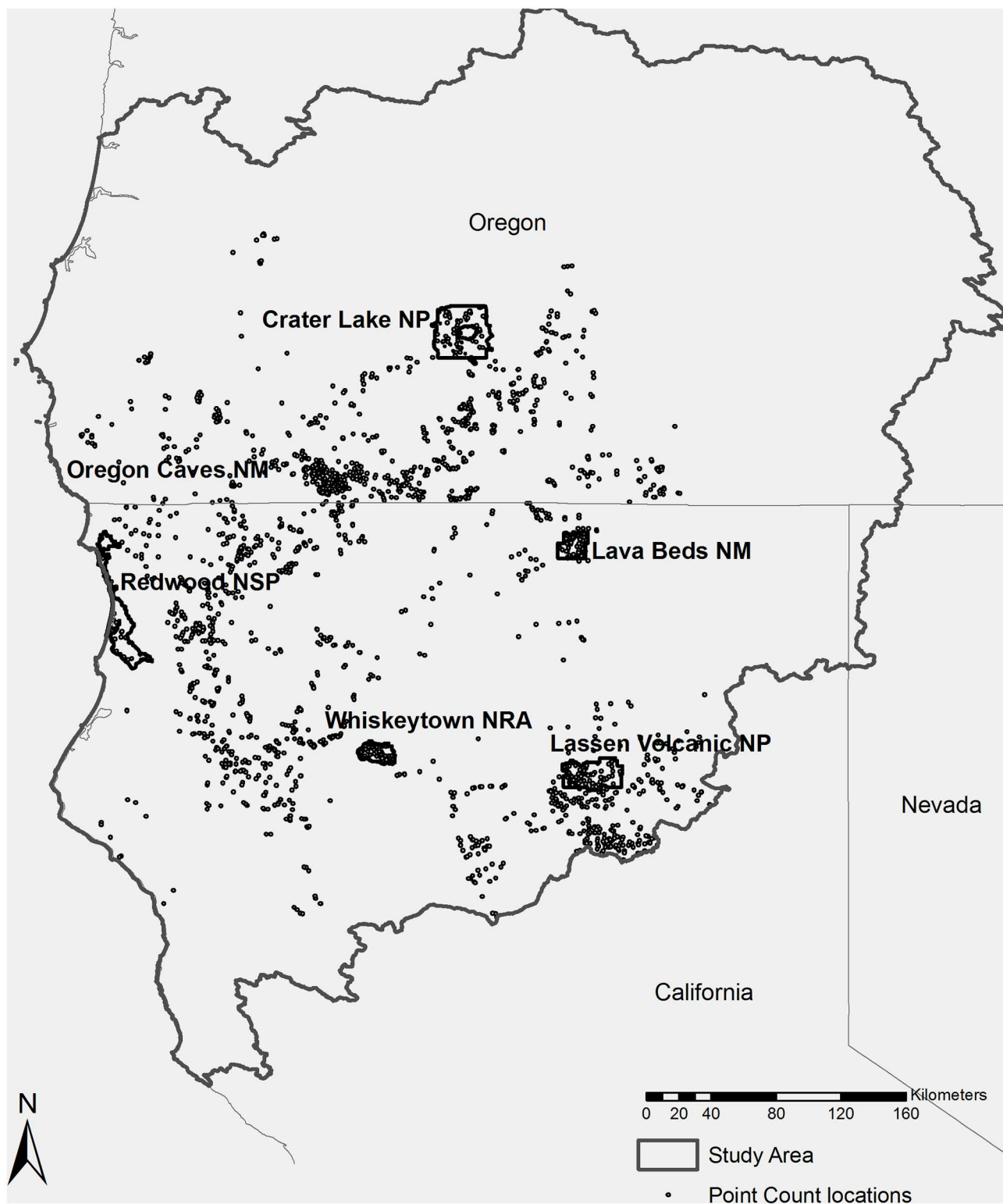
Fig 1. Study Area. The study area is defined by the Klamath Ecoregion located in northern California and southern Oregon. Final analyses included 1990 bird survey points (see methods ); 259 were located within the six National Park Service park units.
