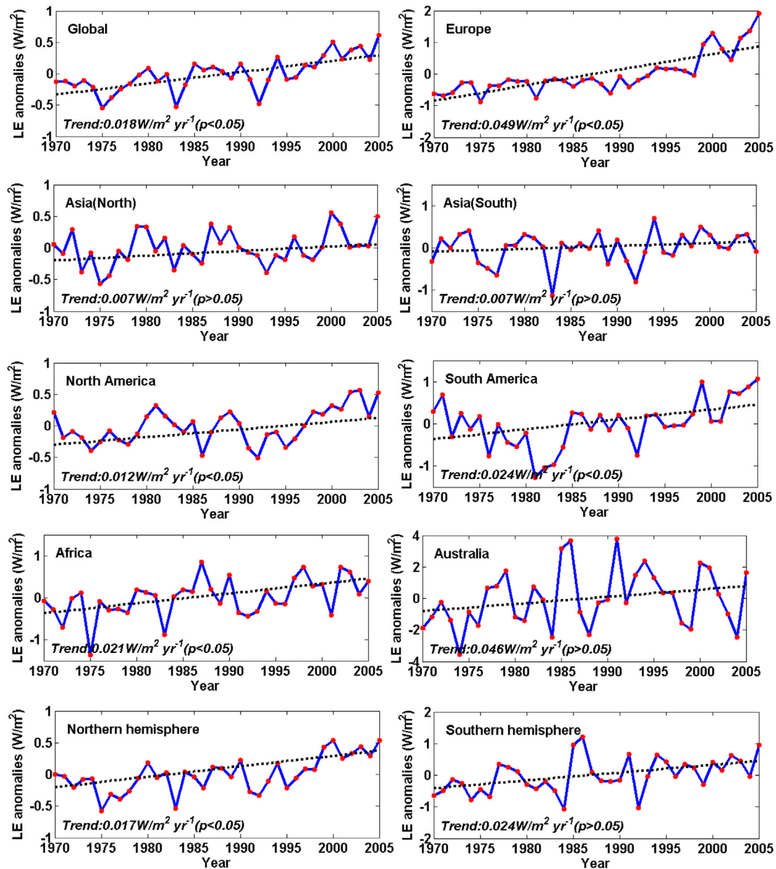
Fig. 11. Regional and global land surface averaged annual LE anomalies. The dashed lines refer to the linear trends in the merged LE based on the BMA method. Unit: \text{W/m}^2 per year.
