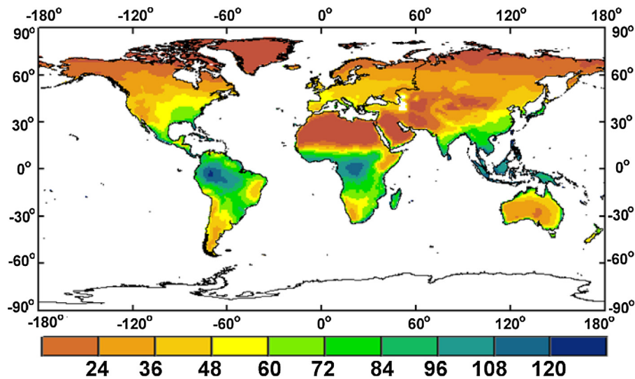
Fig. 9. Spatial distribution of the annual global terrestrial LE averaged for 1970–2005 at a spatial resolution of 1^\circ from the BMA method driven by seven CMIP5 GCMs. Unit: \text{W/m}^2 .
