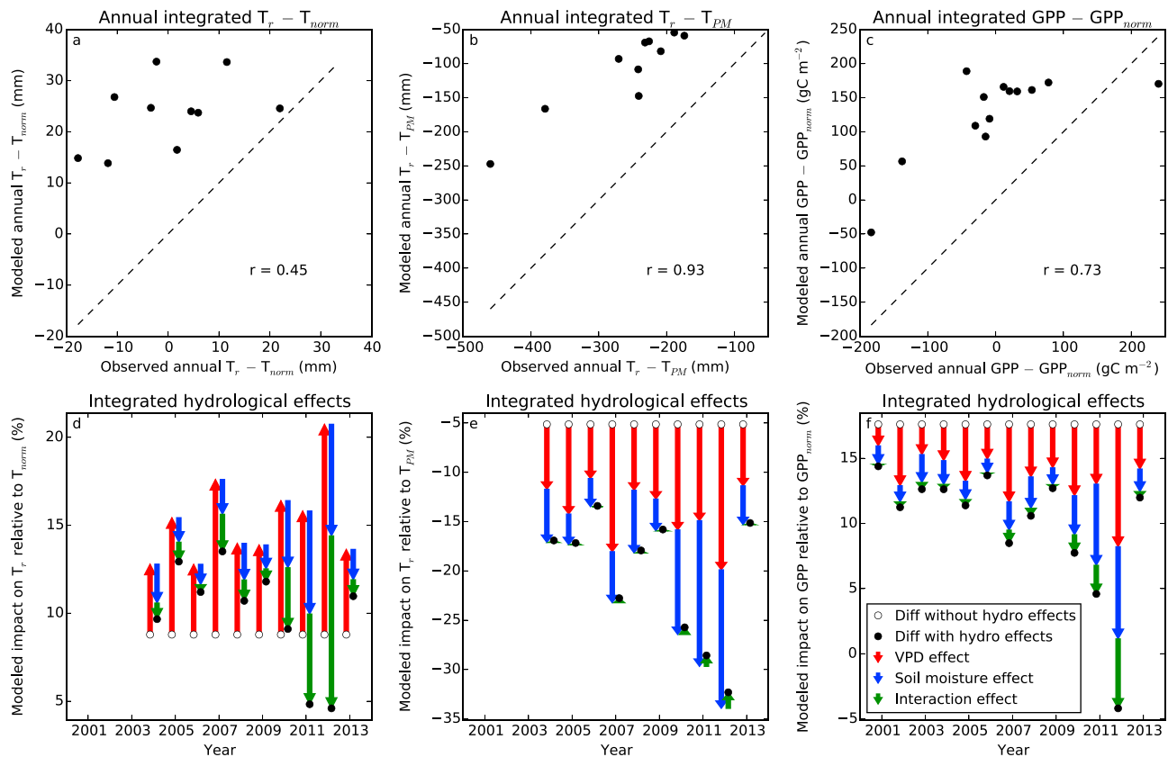
Figure 2. Interannual variations in fluxes and fractions attributed to different hydrological drivers by the statistical model. (a–c) Modeled ( \Delta F_{\text{mod}} ; equation (4)) and observed ( \Delta F ; equation (3)) annual integrated difference between T_r and T_{\text{norm}} (Figure 2a), T_r and T_{PM} (Figure 2b), and GPP and GPP_{\text{norm}} (Figure 2c). Dashed lines show 1-1 relationships. (d–f) Annual integrated contribution of each statistical model term to variations in T_r relative to T_{\text{norm}} (Figure 2d), T_r relative to T_{PM} (Figure 2e), and GPP relative to GPP_{\text{norm}} (Figure 2f). Red, blue, and green arrows show effects of VPD, soil moisture, and their interaction, respectively (equations (6)–(8)). White circles show \Delta F_{\text{Intercept}} (equation (5)). Black circles show the combined effect of all statistical model terms (equivalent to \Delta F_{\text{mod}} ). When this total is greater than zero, the integrated modeled flux is greater than the integrated multiyear mean flux.
