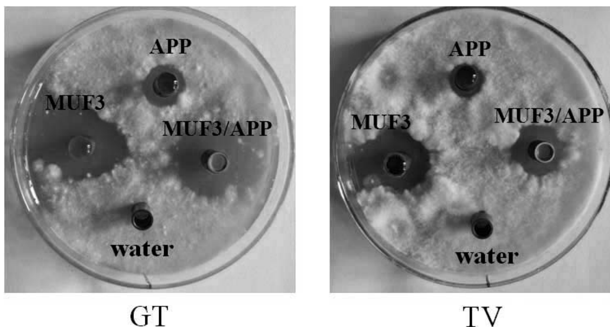
Figure 1.—The decay fungus inhibition test for melamine-modified urea-formaldehyde resin type 3 (MUF3), ammonium polyphosphate (APP), and MUF3 mixed with APP (MUF3/APP); GT = Gloeophyllum trabeum (Pers. ex Fr.); TV = Trametes versicolor (L. ex Fr.).
