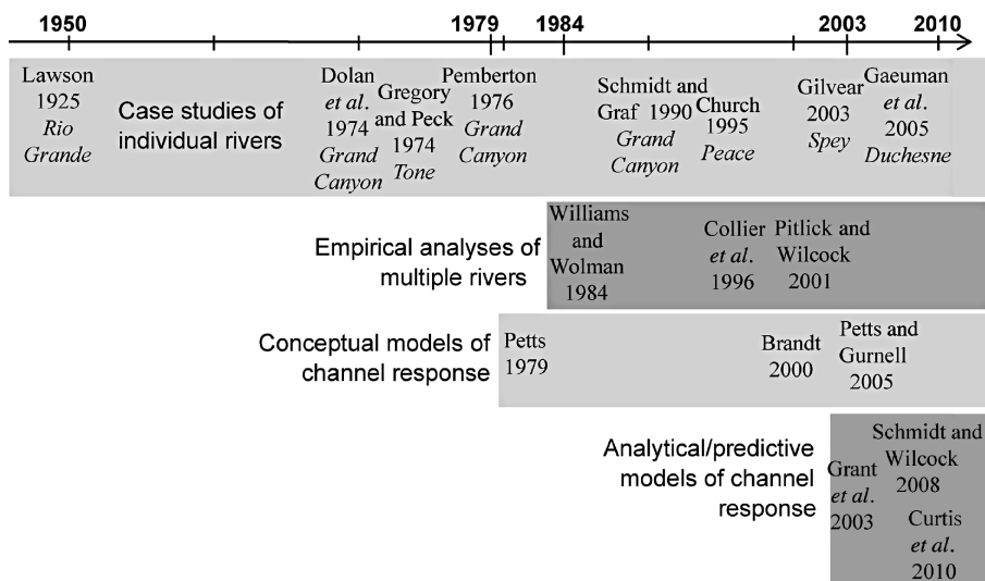
Figure 15.2 Chronology of primary approaches for examining geomorphic response of rivers to dam removal highlighting keystone or representative papers.
