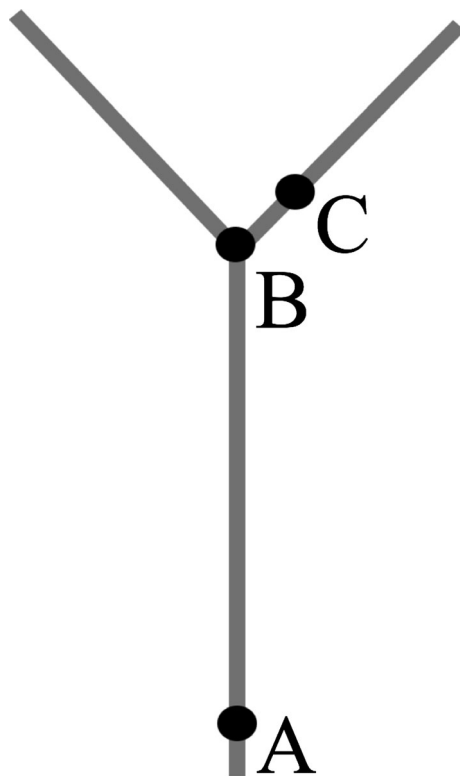
Fig. 1 Reference points for recording time to trail (seconds from A to B ), time to choice (seconds from B to C ), and total assay time (seconds from A to C ), where points represent the beetle's location on a Y-twig during each assay
