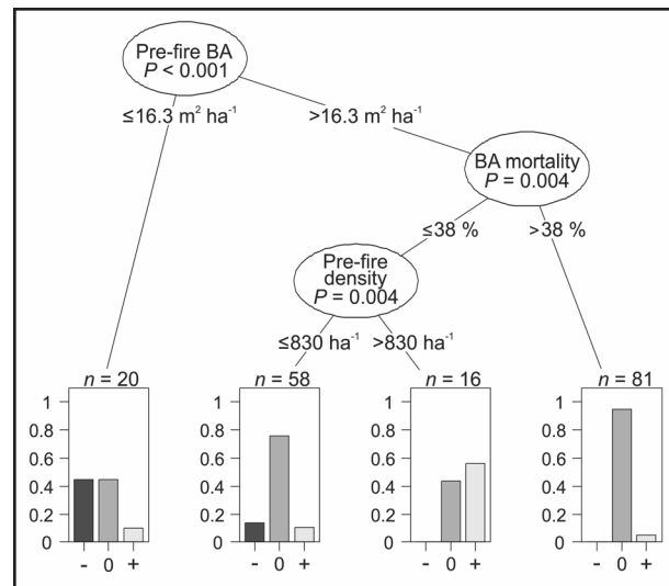
Figure 4. Classification tree depicting the relationships between initial and extended assessment severity categories for the 2013 Rim Fire in Stanislaus National Forest, USA. Minus (plus) sign represents plots that were classified at a lower (higher) severity level in the extended assessment as compared to the initial assessment, and 0 represents plots with no change in severity category. The y-axis shows proportion of plots in each tree node. BA is basal area.
