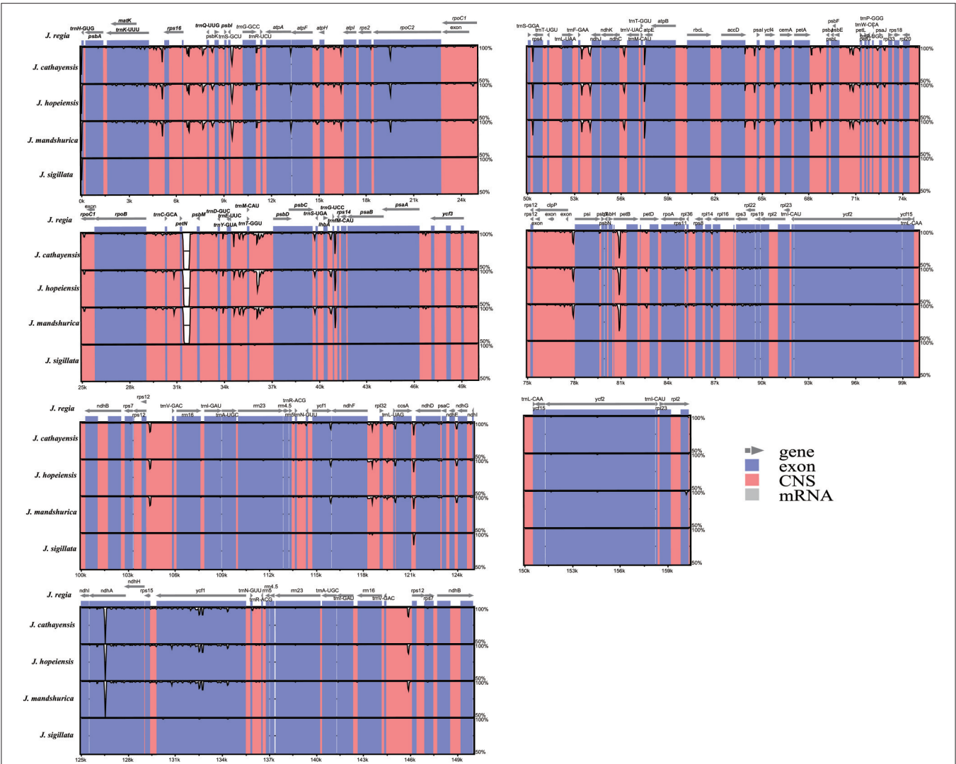
FIGURE 3 | Sequence identity plot comparing the five Juglans chloroplast genomes with J. regia as a reference by using mVISTA. Vertical scale indicates the percentage of identity ranging from 50 to 100%. Coding regions are marked in blue and non-coding regions are marked in red. Gray arrows indicate the position and direction of each gene.
