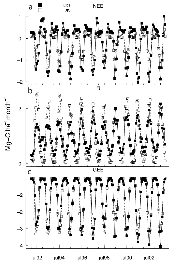
Figure 14. Monthly averages of (a) NEE, (b) R (b), and (c) GEE are shown for IBIS-2 predictions (open symbols with dashed line) and compared to observations (solid symbols).
