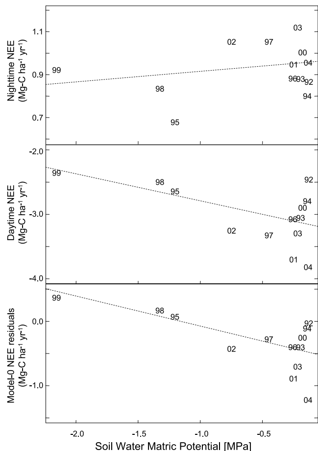
Figure 12. Midsummer (DOY 206–250) NEE and Model-0 NEE residuals versus simulated midsummer mean soil water matrix potential. YY markers denote year (e.g., 99 = 1999). NEE is in units of \text{Mg-C ha}^{-1} \text{ yr}^{-1} ; matric potential is in units of MPa. (top) Observed nighttime NEE. (middle) Observed daytime NEE, R^2 = 0.32 , t = -1.55 ; the correlation is statistically significant at the 90% confidence level. (bottom) Model-0 NEE residuals (observed – predicted), R^2 = 0.45 , t = -2.42 ; the correlation is statistically significant at the 95% confidence level. Soil water matrix potential was estimated using the bucket hydrology model simulated volumetric soil moisture and water retention curves for Harvard Forest [Savage and Davidson, 2001].
