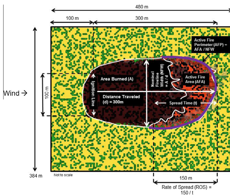
Fig. 8. Schematic summary of FIRETEC simulation analysis metrics. Four metrics were derived from each simulation: area burned, rate of spread, nominal fireline width and active fire perimeter and all metrics were compared between pairs of simulations for dormant and spring dip conditions.
