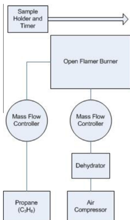
Fig. 1. Flow diagram of the open-flame igniter apparatus.
