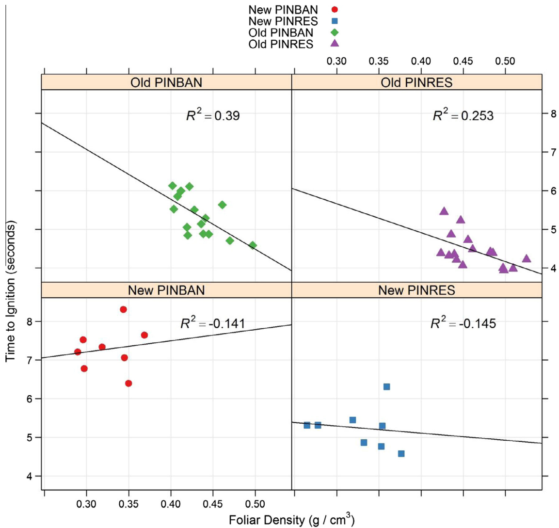
Fig. 6. Relationship between foliar density and time to ignition for new and old foliage of Jack pine (PINBAN) and Red pine (PINRES). Ignition time was most influenced by foliar density in old foliage of both species and was less pronounced in new foliage.
