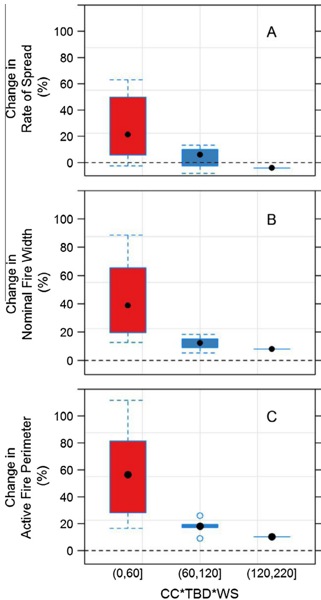
Fig. 9. Summary of changes in FIRETEC-modeled rate of spread (A), nominal fireline width (B) and active fire perimeter (C) between dormant and spring dip conditions plotted against the product of canopy cover (CC), within-tree bulk density (TBD) and wind speed (WS). For all variables as CC, TBD and/or WS increases, the influence of the dip on simulated fire behavior diminishes.
