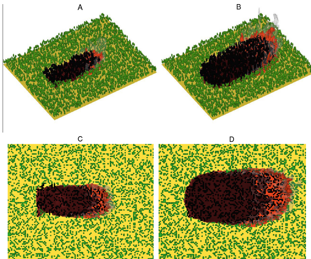
Fig. 7. Comparison of the area burned over the same simulation time (280 s) for the moderate density ( 0.22 \text{ kg m}^{-2} ), low canopy cover (30%) and low windspeed case ( 4.2 \text{ m s}^{-1} ) for dormant season conditions (A and C) and spring dip conditions (B and D).
