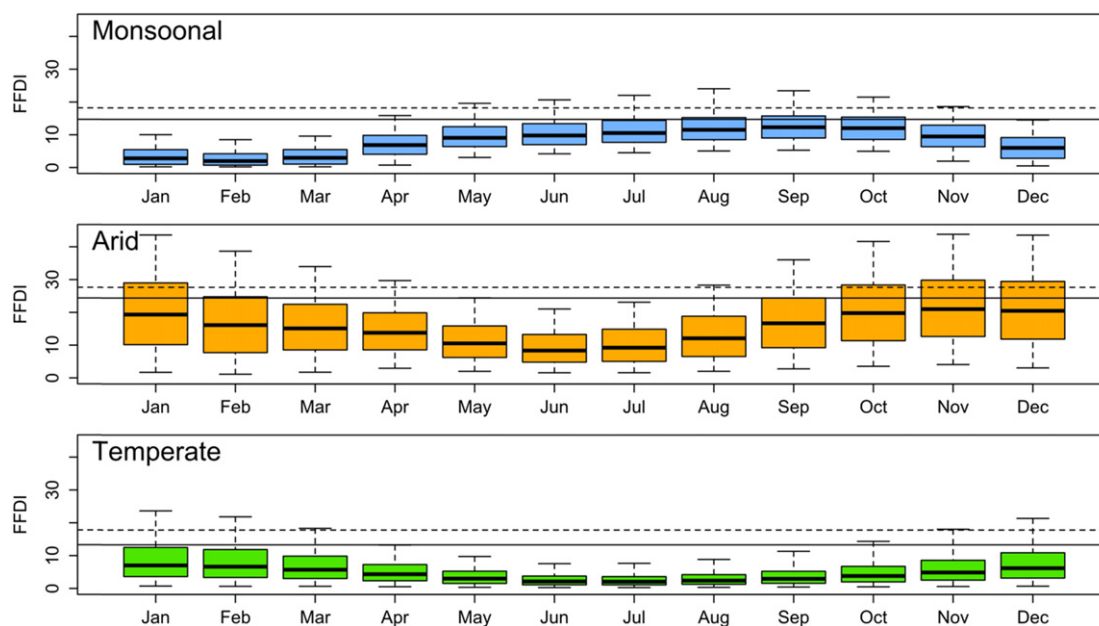
Figure 4. Variability in area-weighted regional mean daily FFDI values for each calendar month in each climate zone. Boxes span the 25th–75th percentiles, the line within the box shows the median, while whiskers indicate the 5th and 95th percentiles of the data. The solid horizontal line indicates FFDI 50 (the median FFDI for day-time hotspots) for that climate zone, and the dashed line represents the night-time FFDI 50 .
