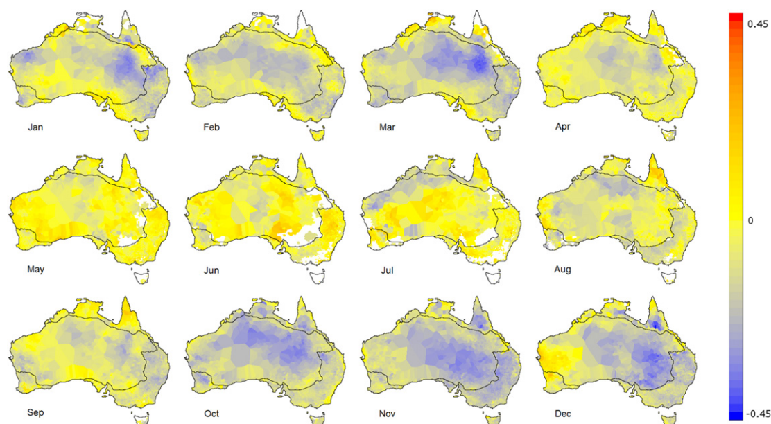
Figure 5. Correlations between the proportion of days above FFDI 50 and Southern Oscillation index (SOI). Maps show the spatial pattern of the Pearson correlation coefficient for the proportion of days in each month above FFDI 50 for that climate zone versus the 12 month running mean SOI for 1900–2011. FFDI 50 is the median FFDI on days with recorded fire activity. White polygons indicate there were too few days above the threshold for a correlation to be calculated. Note that negative values of SOI are associated with hot, dry conditions over much of Australia, leading to the observed negative correlations with FFDI (shown in blue).
