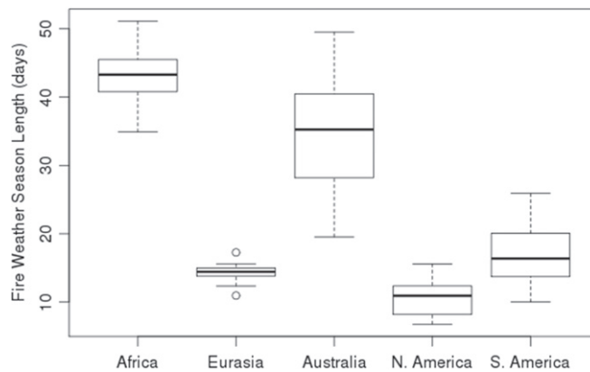
Figure 2. Global comparisons of area-weighted mean fire season length by continent, based on analyses of the dataset of Jolly et al (2015) where fire season length is defined in their work as the number of days each year when fire danger is above half its value range. Analyses for biomes within continents are shown in appendix S5.
