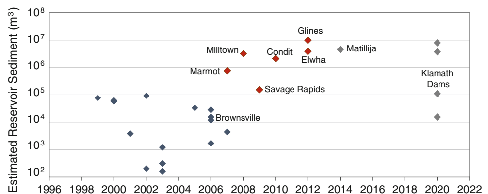
Fig. 7.1 Estimated reservoir sediment stored behind selected dams prior to removal. (Major et al. 2012; unpublished data)
