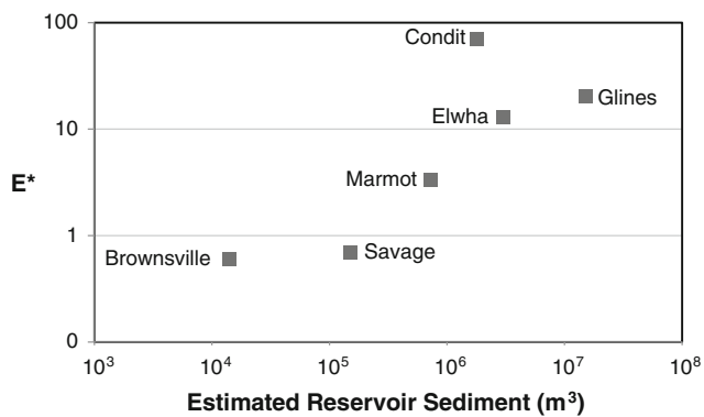
Fig. 7.3 Fraction of stored sediment eroded in the first year after dam removal relative to the background sediment flux ( E^* ) for selected recent dam removals in the Pacific Northwest
