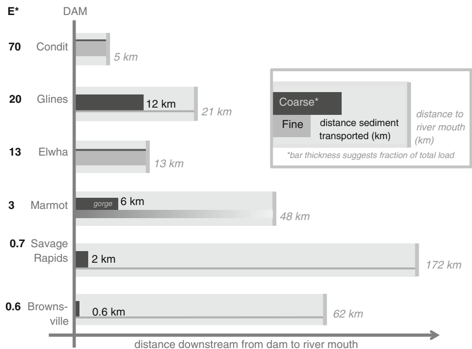
Fig. 7.4 Approximate transport distances for sediment released following dam removal for both fine and coarse fractions. Sites are organized from top to bottom by decreasing first-year calculated E^* . Bar thickness represents relative fraction of each grain size class in the initial reservoir deposit. (O'Connor et al. 2001; Sawaske and Fryburg 2012; Stewart and Grant 2005; Walter and Tullos 2012; unpublished data)
