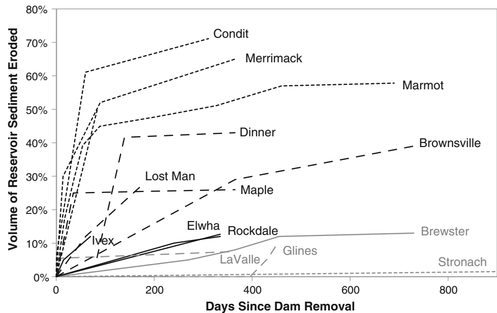
Fig. 7.2 Patterns of sediment evacuation after staged (gray shading) or rapid (black lines) dam removal. General sediment size and cohesiveness is indicated by line type as follows: Solid cohesive, fine sediments, long dash gravel, short dash >55 % sand. (O'Connor et al. 2001; Sawaske and Fryburg 2012; Stewart and Grant 2005; Walter and Tullos 2012)
