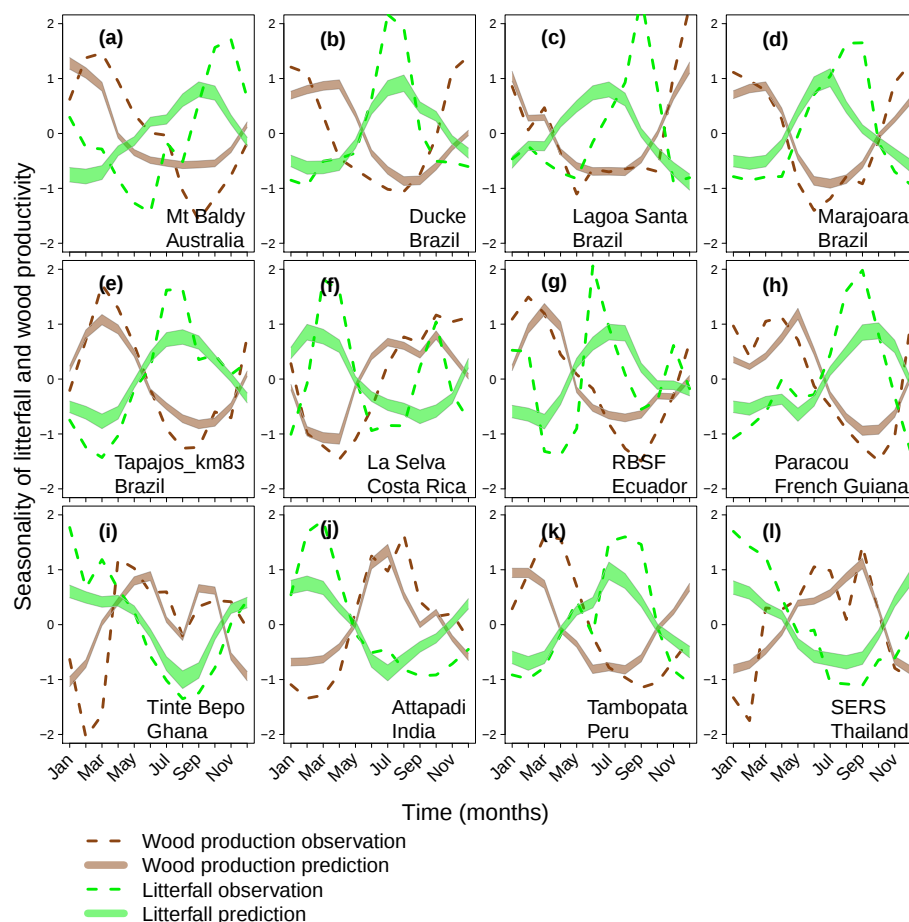
Figure 9. Observations and predictions of wood productivity and litterfall seasonality in sites where both measurements were available. The outliers in our analysis, Lambir and Caracai, are not represented. y axis have no units as the variables were normalized.
