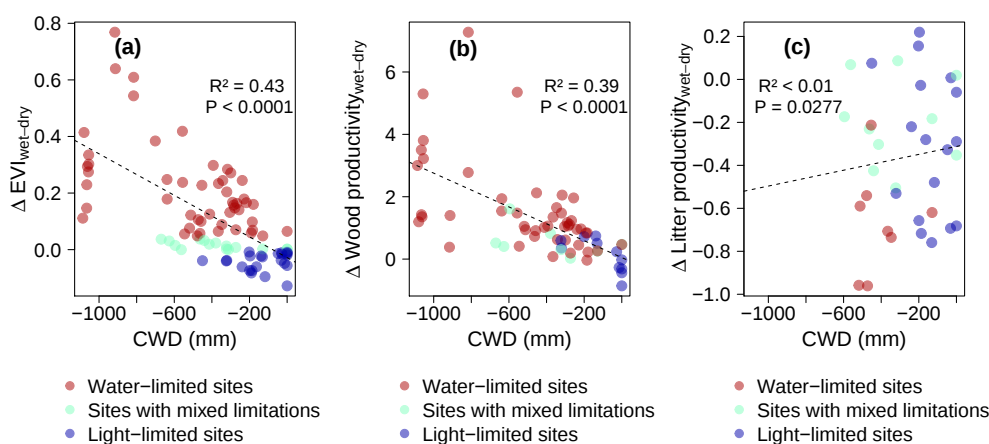
Figure 11. Associations between site's \Delta \text{EVI}_{\text{wet-dry}} (a), \Delta \text{wood productivity}_{\text{wet-dry}} (b) and \Delta \text{litter productivity}_{\text{wet-dry}} (c) with the environmental variable maximum climatological water deficit (CWD). Dashed lines are the regression lines. \Delta \text{EVI}_{\text{wet-dry}} , \Delta \text{wood productivity}_{\text{wet-dry}} and \Delta \text{litter productivity}_{\text{wet-dry}} indices are the differences of mean of the wet- and dry-season of the variable normalized by the annual mean, where dry season is defined as months with potential evapotranspiration above precipitation (Guan et al., 2015). For the sites where evapotranspiration is never above precipitation, dry season is defined as months with normalized potential evapotranspiration above normalized precipitation.
