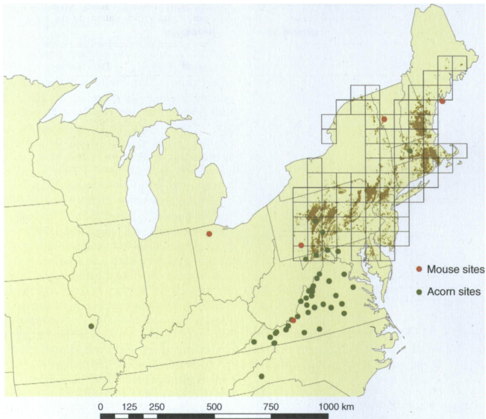
FIG. 1. Source locations of red oak acorn ( Erythrobalanus ), white-footed mouse ( Peromyscus leucopus ), and gypsy moth ( Lymantria dispar ) abundance data sets. For each forest quadrat (black outlined squares), the percentage of forest canopy defoliated was used as a proxy of gypsy moth abundance in a given year. Areas defoliated by gypsy moths between 1975 and 2005 are marked in brown.
