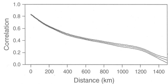
FIG. 6. The spatial correlation function estimated from simulated weather conditions. The upper and lower lines represent 95% bootstrap confidence intervals. The correlation function of the simulated weather conditions closely matches that of temperature and precipitation data for the gypsy moth's range in North America (see Peltonen et al. 2002: Fig. 2).
