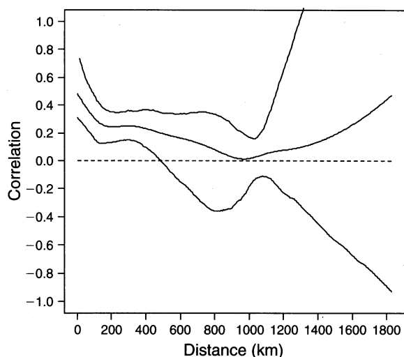
FIG. 2. The spatial correlation function of red oak acorn density data. The upper and lower lines represent 95% bootstrap confidence intervals.
