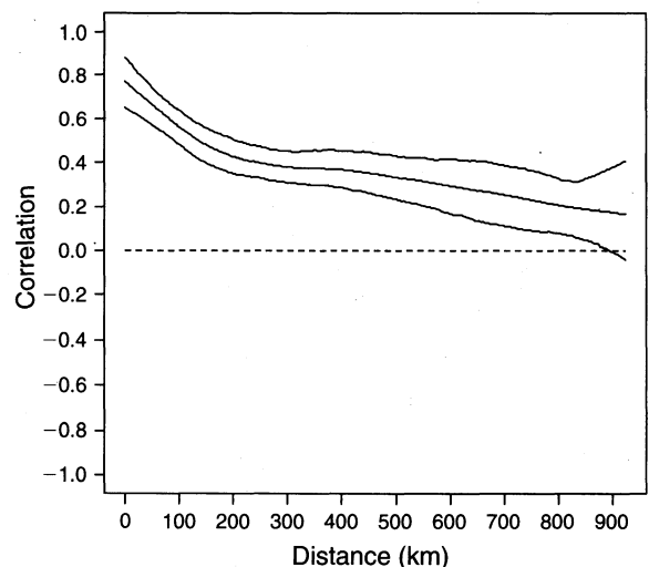
FIG. 4. The spatial correlation function from gypsy moth defoliation data. The upper and lower lines represent 95% bootstrap confidence intervals.
