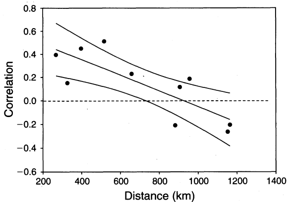
FIG. 3. Relationship between population synchrony (correlation) and distance estimated from white-footed mouse data. The upper and lower lines represent 95% confidence intervals.
