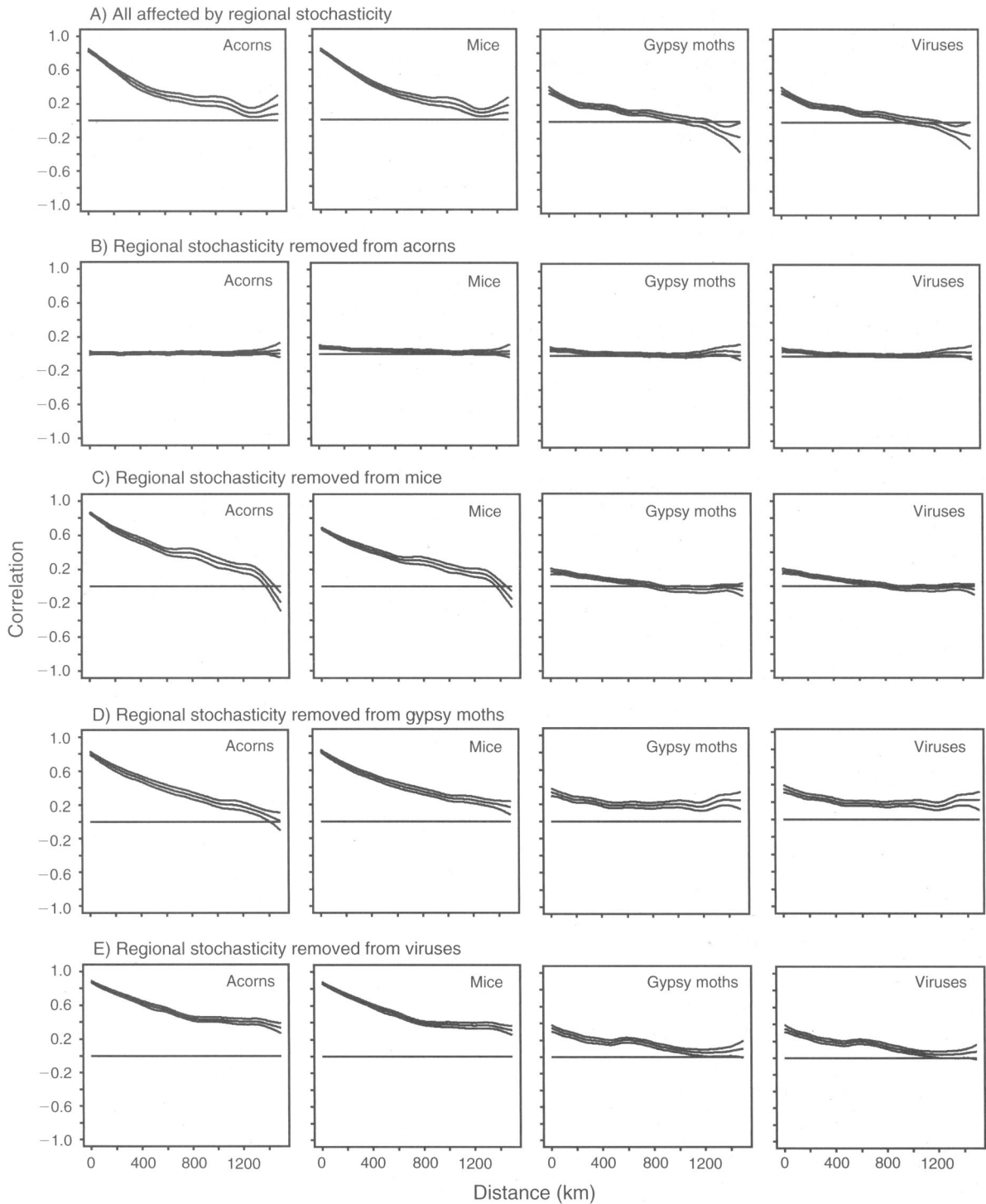
FIG. 5. The spatial correlation functions estimated from models with (A) regional stochasticity affecting each species, (B) no regional stochasticity affecting acorns, (C) no regional stochasticity affecting white-footed mice, (D) no regional stochasticity affecting gypsy moths, and (E) no regional stochasticity affecting the pathogen. The upper and lower lines represent 95% bootstrap confidence intervals.
