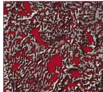
Figure 12—Inversion on the intermountain domain of the United States.
