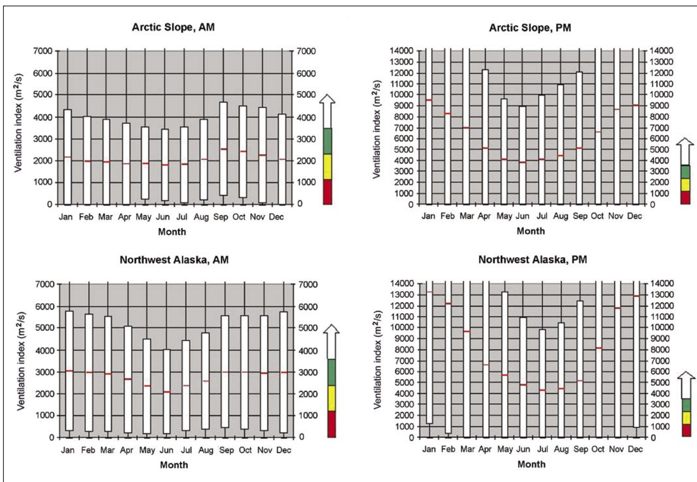
Figure 24—Box plots of ventilation index by month for each regional airshed in Alaska. Color bars to the right of each plot indicate categories of poor (red), marginal (yellow), fair (green) and good (white) ventilation potential.
