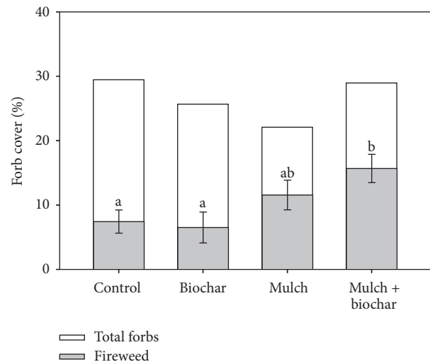
FIGURE 3: Total forb and fireweed ( Chamerion angustifolia ) cover in August 2016, the third season after post-fire rehabilitation treatment establishment at the Church's Park burn, Colorado. Bars show means and standard errors for fireweed sampled in six replicate treatment blocks. Letters denote significant differences among fireweed cover means at \alpha = 0.05 level.
