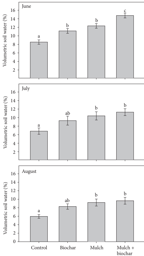
FIGURE 2: Volumetric soil water content (0–10 cm depth) under post-wildfire rehabilitation treatment at the Church's Park burn, Colorado. Soil water was measured at 6 replicate blocks of treatments, 6 times per year during 2014, 2015, and 2016. Bars show means and standard errors of six replicate treatment blocks. Letters denote significant differences among means at \alpha = 0.05 level.
