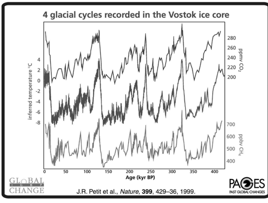
Figure 17-1. Primary fluctuations in temperature, \text{CO}_2 , and \text{CH}_4 between glacial and interglacial periods for the past 400,000 years, derived from oxygen-isotope analysis of ice cores from the Vostok station in Antarctica. Our current interglacial period (Holocene) is at the far left , from 0 to 10,000 years ago. Pages International Project Office—modified from Petit et al. 1999.
