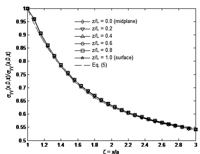
Fig. 7. Variations in stress ratio \sigma_{yy}(x, 0, z)/\sigma_{yy}(a, 0, z) for x/a \geq 1 on different lateral planes ( x, 0, z/L ) in Sitka spruce for thickness L/a = 5 when longitudinal axis (grain orientation, L -direction) is perpendicular to applied vertical stress, \sigma
