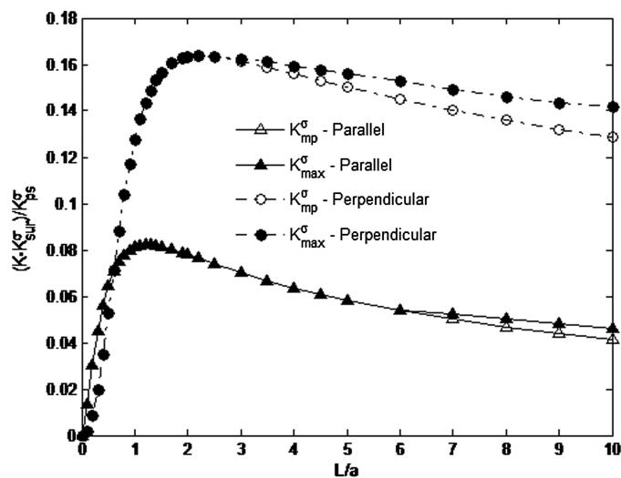
Fig. 14. Differences between the normalized midplane, (K_{mp}^\sigma - K_{sur}^\sigma)/K_{ps}^\sigma , and maximum, (K_{max}^\sigma - K_{sur}^\sigma)/K_{ps}^\sigma and surface stress concentration factors in Sitka spruce as a function of normalized plate thickness L/a when the grain orientation is parallel and perpendicular to applied vertical stress, \sigma
