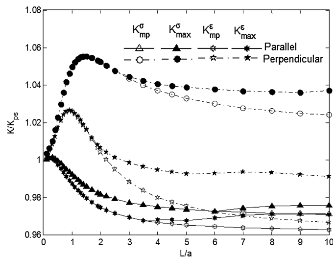
Fig. 12. Distributions of normalized midplane ( K_{mp}^\sigma/K_{ps}^\sigma and K_{mp}^\varepsilon/K_{ps}^\varepsilon ) and maximum ( K_{max}^\sigma/K_{ps}^\sigma and K_{max}^\varepsilon/K_{ps}^\varepsilon ) stress and strain concentration factors in Sitka Spruce as function of plate thickness L/a for different grain orientations (parallel—solid line and perpendicular—dashed line) to applied vertical stress, \sigma
