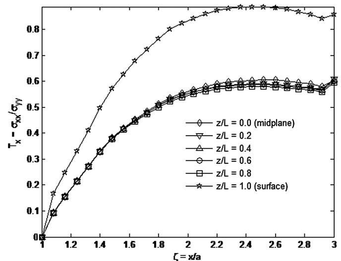
Fig. 6. Variations in stress constraint factor, T_x , for x/a \geq 1 on different lateral planes ( x, 0, z/L ) in Sitka spruce for thickness L/a = 5 when longitudinal axis (grain orientation, L -direction) is perpendicular to applied vertical stress, \sigma
