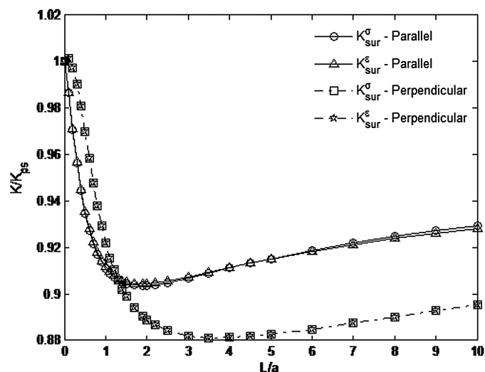
Fig. 13. Distributions of normalized external traction-free surface stress, K_{sur}^\sigma/K_{ps}^\sigma , and strain, K_{sur}^\varepsilon/K_{ps}^\varepsilon , concentration factors in Sitka spruce as function of plate thickness L/a for different rain orientations (parallel—solid line and perpendicular—dashed line) to applied vertical stress, \sigma
