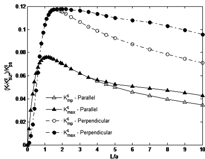
Fig. 15. Differences between the normalized midplane, (K_{\text{mp}}^{\epsilon} - K_{\text{sur}}^{\epsilon})/K_{\text{ps}}^{\epsilon} , and maximum, (K_{\text{max}}^{\epsilon} - K_{\text{sur}}^{\epsilon})/K_{\text{ps}}^{\epsilon} , and surface stress concentration factors in Sitka spruce as a function of normalized plate thickness L/a when the grain orientation is parallel or perpendicular to applied vertical stress, \sigma
