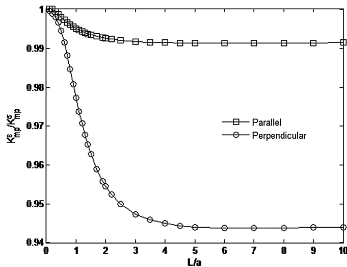
Fig. 18. Distribution of midplane K^\varepsilon/K^\sigma at the edge of the hole in Sitka spruce as a function of thickness when the grain orientation is parallel or perpendicular to applied vertical stress, \sigma
