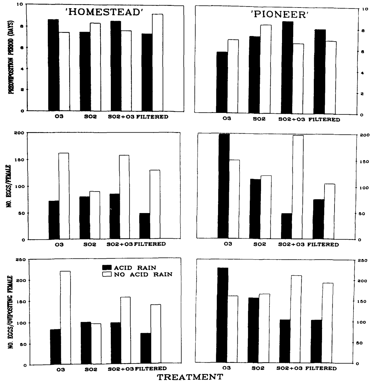
Figure 5. Oviposition during a 2-week period by elm leaf beetles fed leaves harvested from elms exposed for 9 weeks to simulated acid rain, and ozone and sulfur dioxide fumigation treatments.
