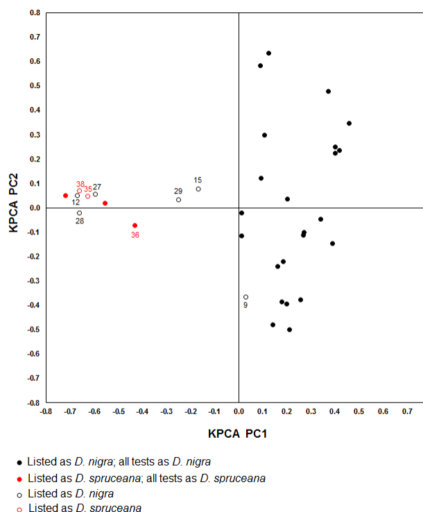
Figure 2. Values of the first two principal components (PC1 and PC2) extracted using kernel principal component analysis (KPCA) for each of the Dalbergia samples analyzed using direct analysis in real time–time of flight mass spectrometry (DART–TOFMS). Numbers above or below open circles refer to sample numbers in Table 2.
