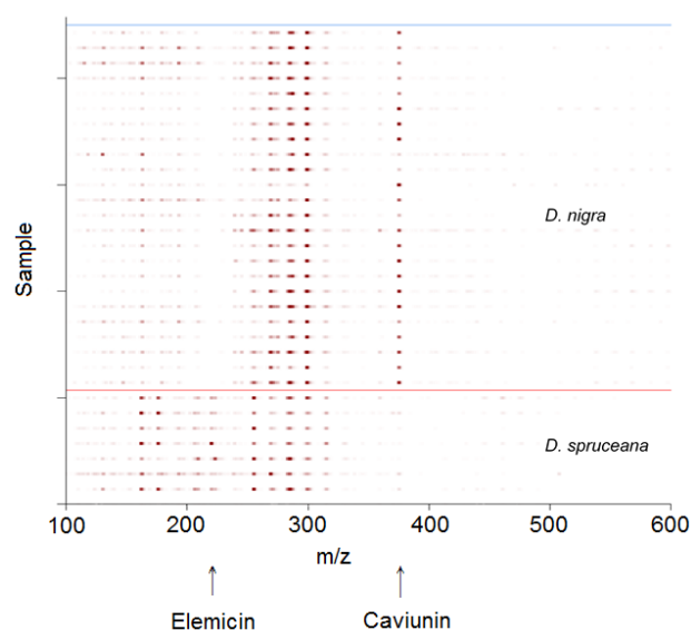
Figure 1. Graphical representation (heat map) of the spectral results comparing the heartwood of Dalbergia nigra (24 samples, between blue line and red line) with that of Dalbergia spruceana (seven samples, below red line). The abscissa, m/z , is the mass-to-charge ratio of the compound detected (its molecular mass divided by its electrical charge), and the ordinate contains the individual samples. The compound elemicin, indicated by the arrow on the left, is prominent in D. spruceana but faint or absent in D. nigra . The compound caviunin, indicated by the arrow on the right, is prominent in D. nigra but faint or absent in D. spruceana .
