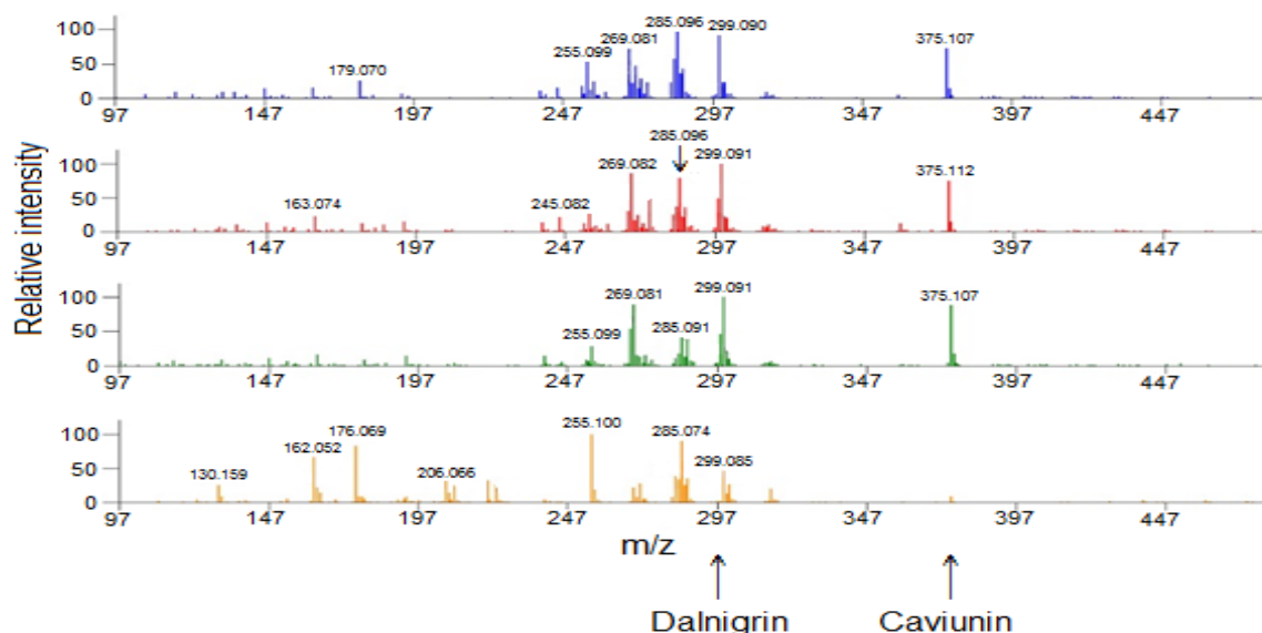
Figure 4. Comparison of direct analysis in real time–time of flight mass spectrometry (DART–TOFMS) mass spectrum of unvouchered Dalbergia nigra sample 9 (top, blue) with the spectra of two vouchered D. nigra samples, sample 1 (second from top, red) and sample 10 (third from top, green), and vouchered sample 35 of D. spruceana (bottom, yellow). Each peak corresponds to an ion that was detected in the wood sample. The abscissa, m/z (mass-to-charge ratio), is the molecular weight of an ion divided by its charge number, and the ordinate is the relative signal intensity of the ions. The compounds dalnigrin and caviunin, found in the D. nigra samples, are indicated by the labelled arrows. In D. spruceana , two much smaller peaks are found at the same m/z values, but these are not dalnigrin or caviunin (Kite and others 2010).
