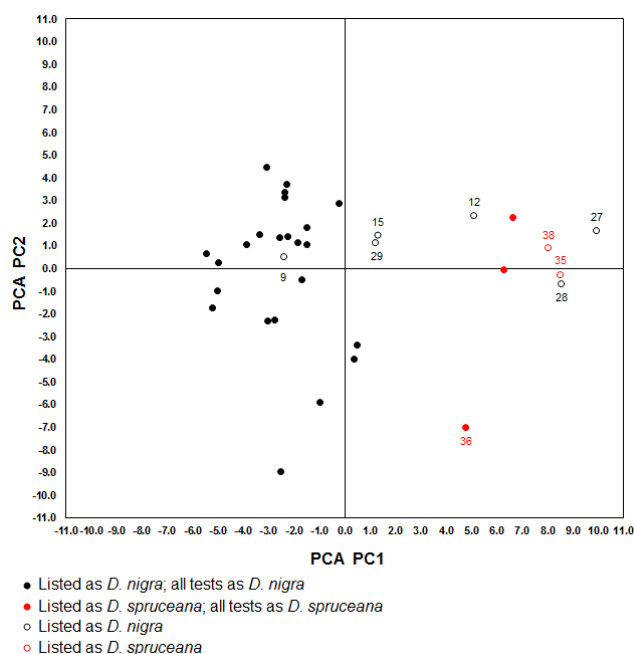
Figure 3. Values of the first two principal components (PC1 and PC2) extracted using principal component analysis (PCA), for each of the Dalbergia samples analyzed using direct analysis in real time–time of flight mass spectrometry (DART–TOFMS). Numbers above or below open circles refer to sample numbers in Table 2.
