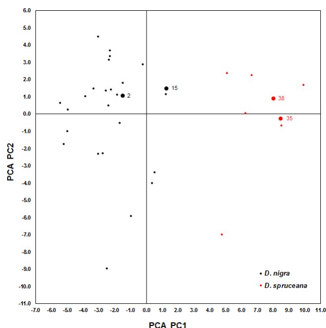
Figure 5. Principal components map for the principal components analysis (PCA) based on the direct analysis in real time–time of flight mass spectrometry (DART–TOFMS) spectra; PCA PC1 is the first principal component, PCA PC2 the second. Large symbols and labels indicate the paired (MAD and SJR) Dalbergia samples. Black symbols are for D. nigra samples, and red symbols are for D. spruceana . Numbers refer to sample numbers in Table 2.
