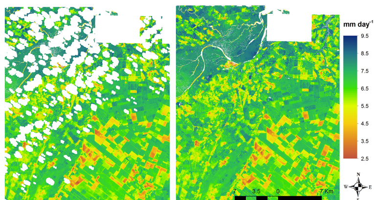
Figure 5. Example of gap-filling cloudy regions in a Landsat 8 ET image for DOY 200. The left image is Landsat-retrieved ET with clouds masked using the Fmask data layer and the right image has been processed through the Landsat gap-filling method.
