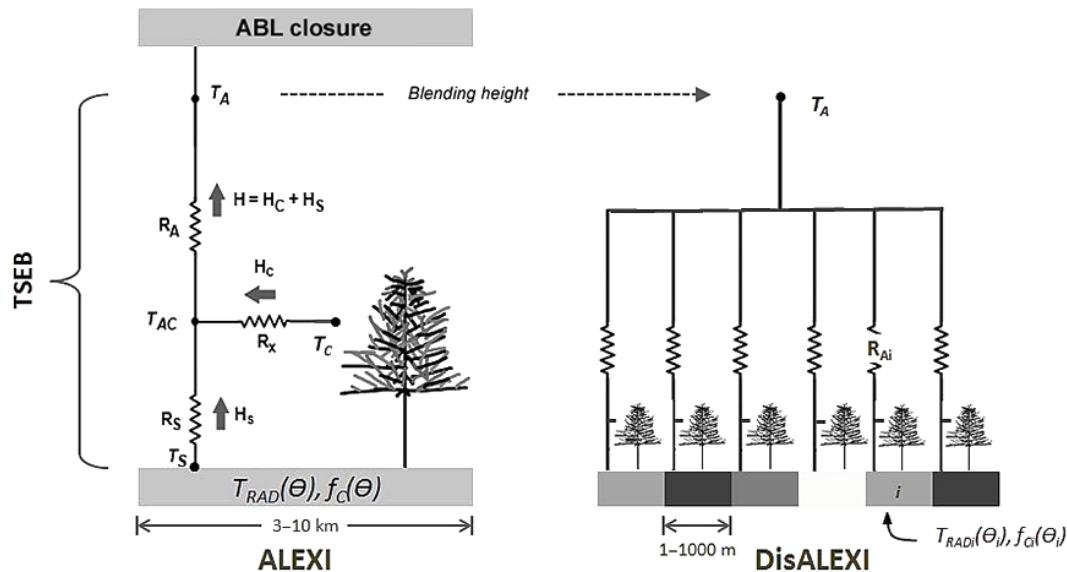
Figure 1. Schematic diagram of the ALEXI and DisALEXI modeling schemes. The left panel shows TSEB as employed to partition the income radiometric temperature ( T_{RAD}(\theta) , \theta is view angle) into canopy (subscript “c”) and soil (subscript “s”) components based on vegetation coverage ( f(\theta) ). Sensible heat ( H ) is regulated by the aerodynamic resistance ( R_A ), bulk leaf boundary layer resistance ( R_x ) and soil surface boundary layer resistance ( R_s ). ALEXI combines the TSEB and ABL models to estimate air temperature ( T_A ) at the blending height. The right panel represents the disaggregation of ALEXI output to finer scales based on LST and f(\theta) information from Landsat and MODIS.
