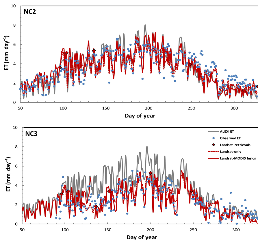
Figure 8. Comparison of time series of ALEXI ET (4 km), observed ET, Landsat ET retrieved on Landsat overpass dates, Landsat-only interpolated ET and Landsat–MODIS fused ET for the NC2 site (and NC3, bottom panel) sites in 2013.
