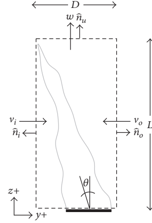
FIGURE 3: Control volume for momentum balance.
