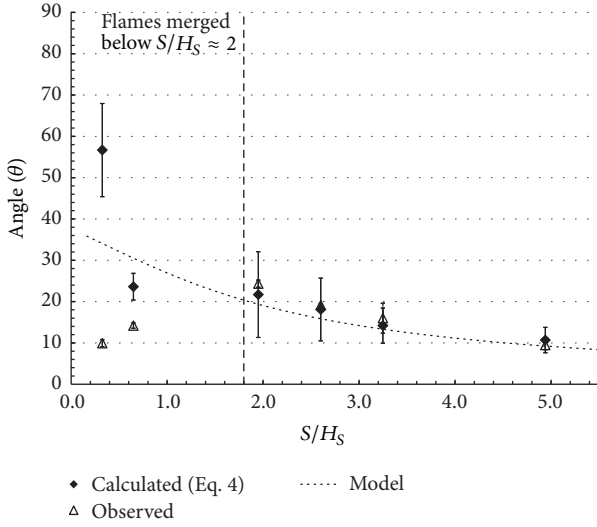
FIGURE 14: Flame angle versus separation distance. Measured value calculated using A = 0.843 . Flames began to merge at spacing below S/H_S = 2 . Error bars represent one standard deviation of the mean. Large uncertainty in measured value is due to the summation of relative uncertainty of the squares of three measured values.
