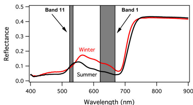
Fig. 1. Needle reflectance spectra of Pinus contorta (lodgepole pine) seedlings in Edmonton, Alberta, Canada, exposed to a boreal winter (red line, March 19, 2013) and summer (black line, June 21, 2013). The positions of MODIS bands 1 and 11 are indicated in gray.
