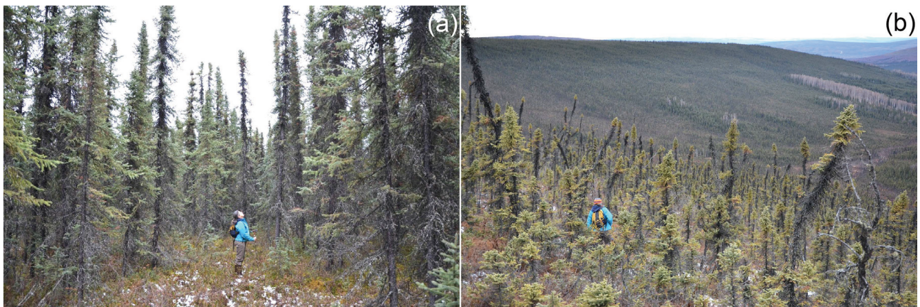
FIGURE 7. The architecture of individual black spruce trees differs widely between sites at Babe Creek: (a) Summit ; and (b) Side slope . These differences likely contribute to the divergent ways these trees respond to climate at both the site- and tree-level .
