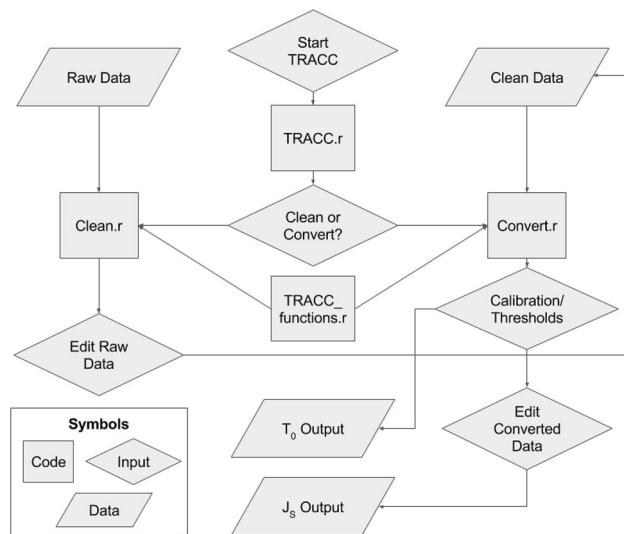
Fig. 1 Flowchart of TRACC software
