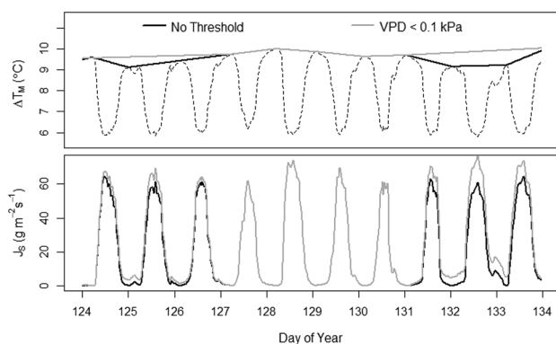
Fig. 2 (Upper panel) Temperature difference measured by probe ( \Delta T_M , dashed) and zero-flow difference ( \Delta T_0 ) estimated with (gray) and without (black) a nightly threshold of 0.1 kPa vapor pressure deficit for 2 h. (Lower panel) Resulting time series of sap flux density ( J_S ) using the two \Delta T_0 estimates
