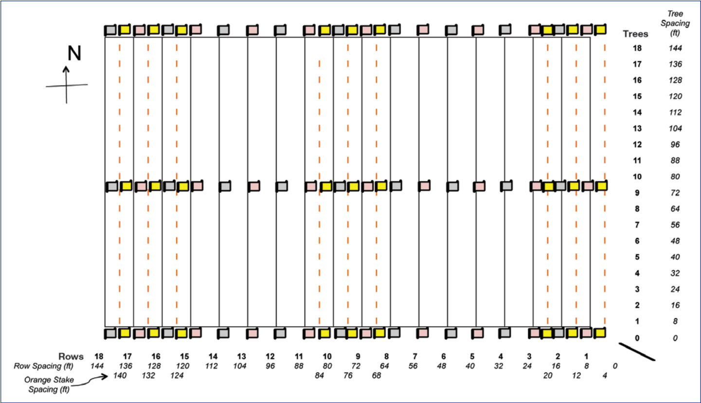
Figure 2. Diagram of the Wright-Michigan State University (W-MSU) method for an 8- by 8-ft plantation containing 324 trees. Three lines of flag stakes on the ends and in the middle of the plantation are baselines the tractor operator will sight on; interior baselines are set at multiples of 8 ft to facilitate marking the orange painted stakes. The orange stakes are positioned in the middle of three rows as indicated; in this example, four rows are skipped and another set of three rows of orange stakes are installed. A string or tape measure is run between the yellow flags on the baseline to mark every 8 ft where the orange stakes are placed.
