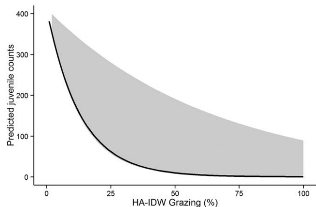
Figure 3. Predicted juvenile blackfish abundance as a function of hydrologically active, inverse-distance-weighted (HA-IDW) grazing (%) in the catchment for an average site, where all predictors included in the final model were held at mean values. Shaded area is 95% confidence interval.
