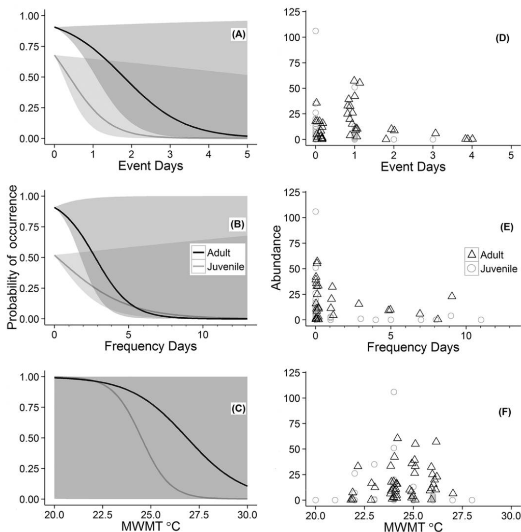
Figure 2. Relationships between probability of occurrence (A–C) and abundance (D–F) of adult and juvenile River Blackfish and the number of successive days stream temperature was >28^{\circ}\text{C} (Event Days) (A, D), the total number of days in summer on which temperature was >28^{\circ}\text{C} (Frequency Days) (B, E), and the highest 7-d moving average of maximum weekly maximum temperature (MWMT) (C, F) estimated from 3 separate hurdle models for an average site where all predictors in the final model were held at mean values. Shaded areas are 95% confidence intervals.
