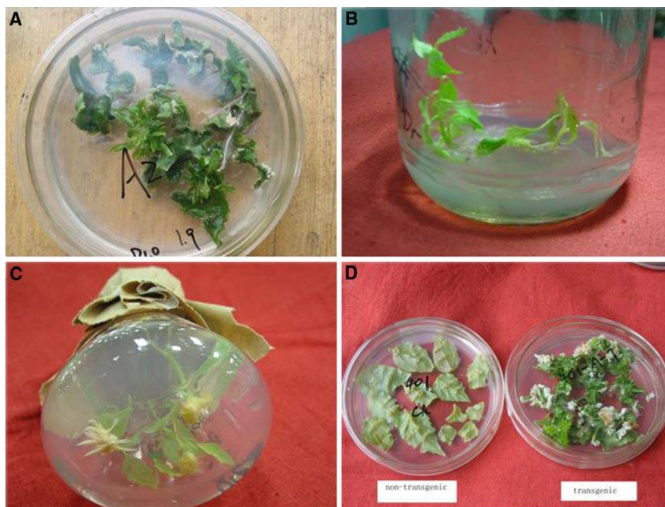
Fig. 2 Adventitious shoot formation and rooting of Populus tomentosa plantlets from transformed leaves. a Adventitious shoot regeneration, b Shoots that survived on initial selection medium containing 30 mg l -1 kanamycin elongated or died on second selection medium with 50 mg l -1 kanamycin, c Rooting of elongated transgenic shoots
