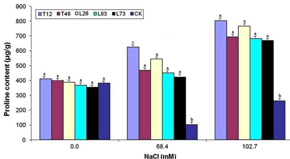
Fig. 5 The effect of 0, 68.4, and 102.7 mM NaCl on leaf proline accumulation for five transgenic plants and a non-transformed control plant. Bars with the same letters are not statistically different ( P < 0.05 )
