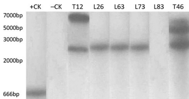
Fig. 4 Southern blot analysis of five transgenic plants of Populus tomentosa for AhDREB1 gene. DNA samples (10 µg) were digested with DraI . + CK positive control, – CK negative control (non-transformed plant), Lanes 3–7 (T12, L26, L63, L73, and L83) putative transgenic plants
