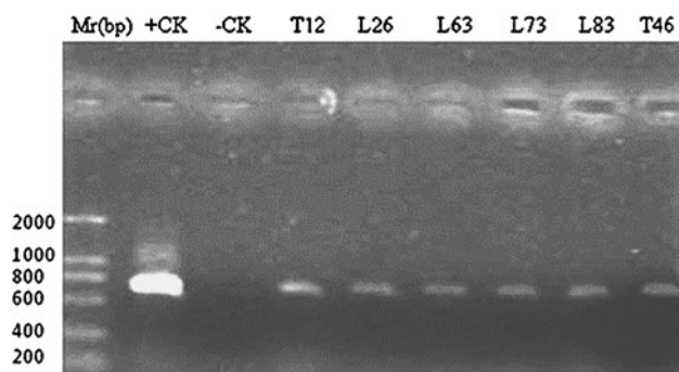
Fig. 3 Polymerase chain reaction analysis of genomic DNA isolated from leaves of non-transformed control and transgenic Populus tomentosa plants using primer pairs specific for amplification of 666 bp AhDREB1 gene. Mr molecular marker, + CK positive control pBI121, – CK negative control non-transformed P. tomentosa , Lanes 4–9 (T12, L26, L63, L73, L83, and T46) putative transgenic P. tomentosa plants
