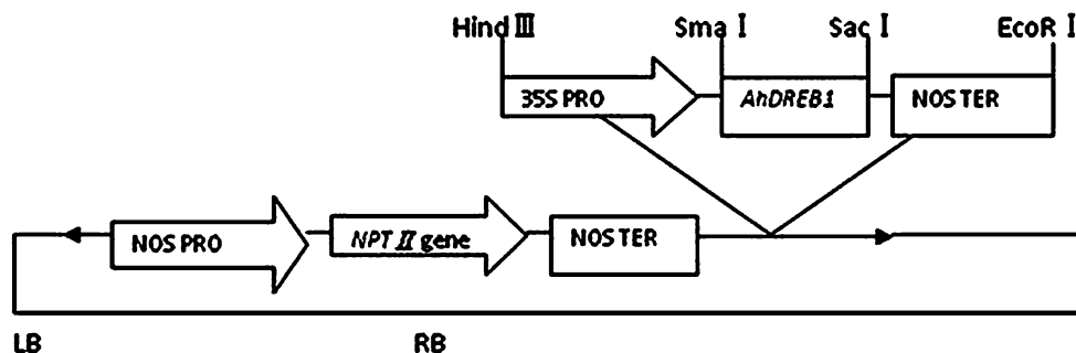
Fig. 1 Schematic diagram of T-DNA region of vector pBI121. LB left border, RB right border, NOS PRO nopaline synthase promoter, NPT II neomycin phosphotransferase II, NOS TER nopaline synthase gene terminator, 35S PRO cauliflower mosaic virus 35S promoter
